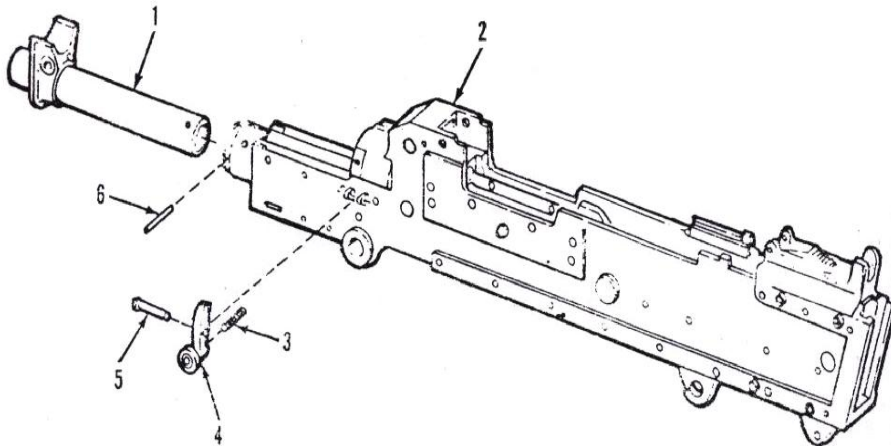
Body, receiver 11826080
