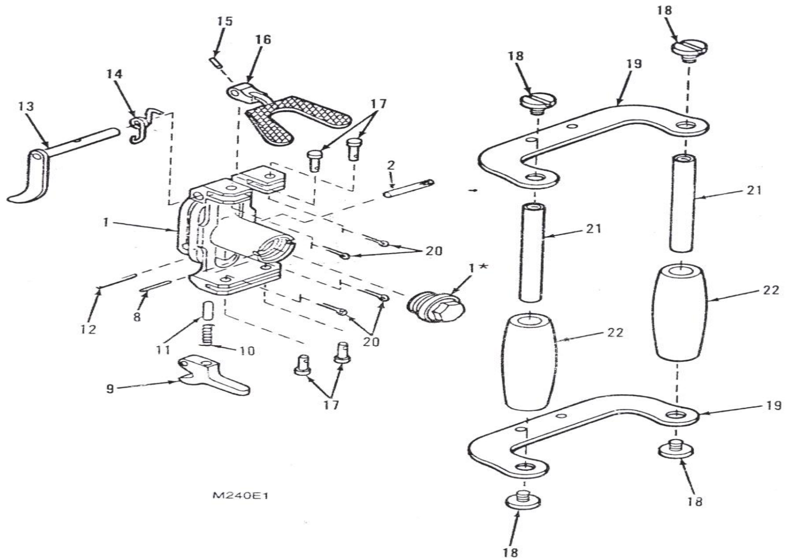
Buffer assembly, M240/M240C 11826211 and buffer and spade grip assembly M240E1 12597057 (Sheet 2 of 2)
