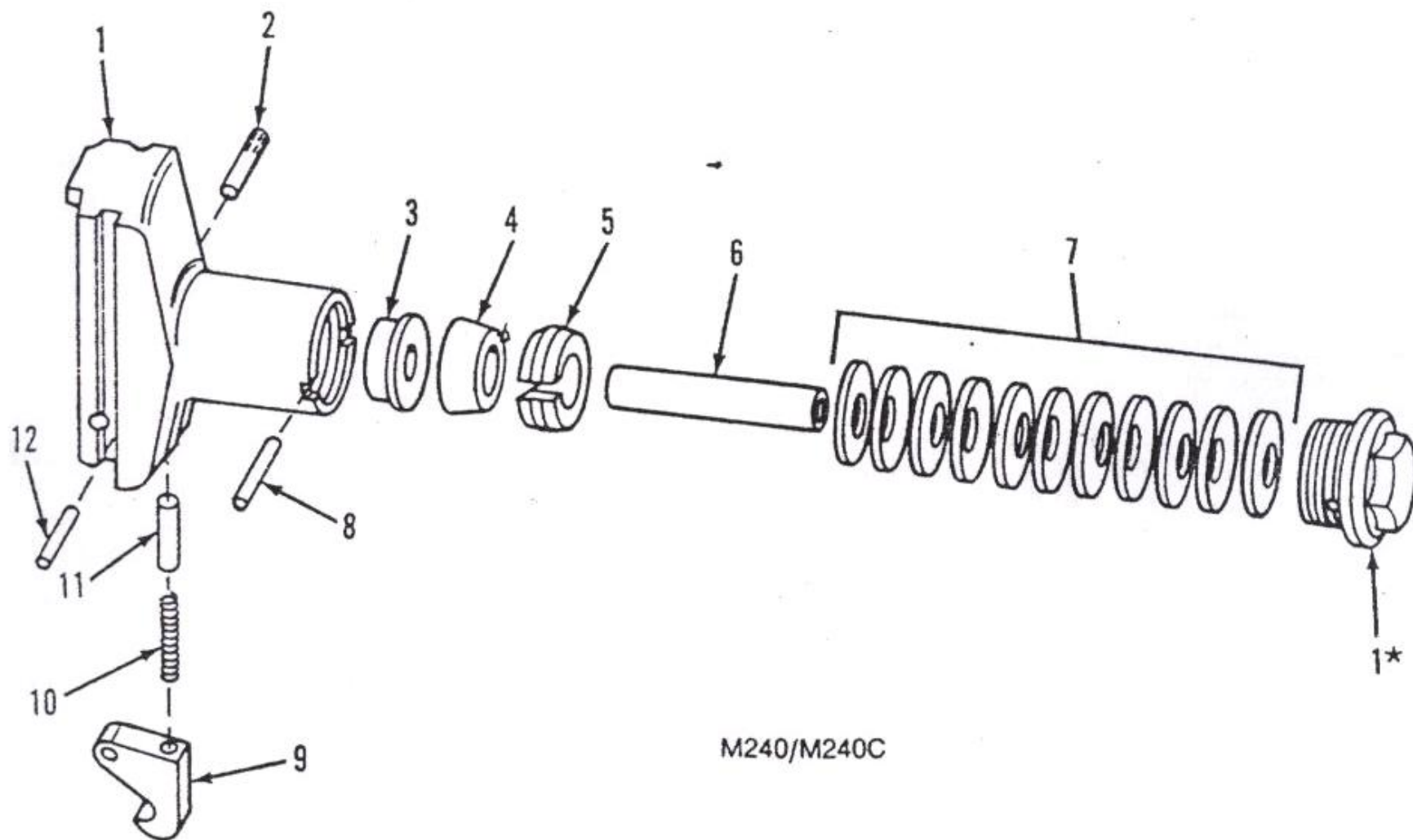
Buffer assembly, M240/M240C 11826211 and buffer and spade grip assembly M240E1 12597057 (Sheet 1 of 2)
