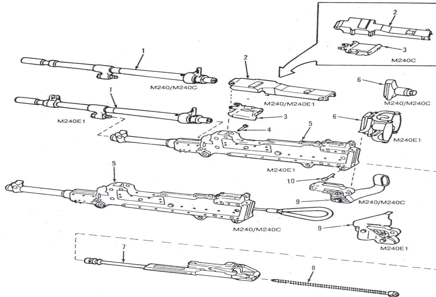
Machine gun, 7.62MM, M240 11825980, M240C 11826004, and M240E1 12597034
