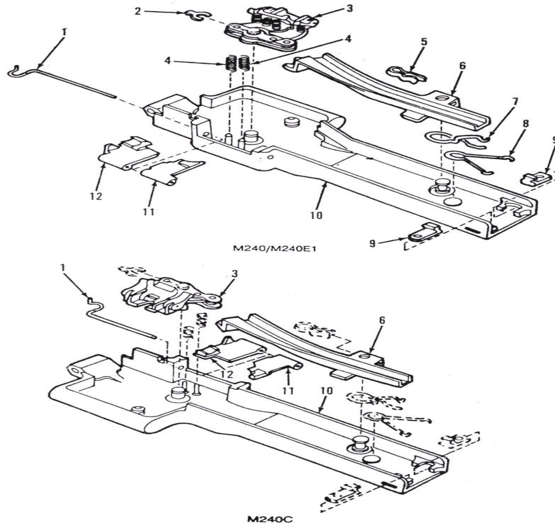
Cover assembly M240/M240E1 11826165 and M240C 11826038
