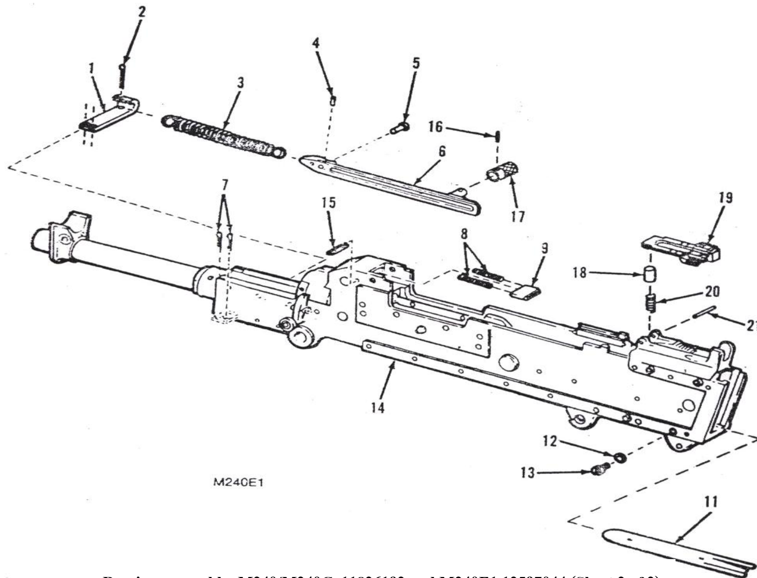
Receiver assembly, M240/M240C, 11826192 and M240E1 12597044 (Sheet 2 of 2)
