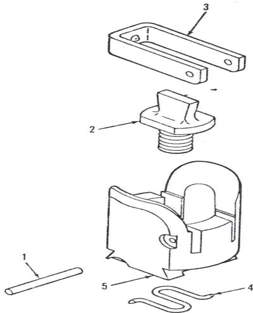
Front sight assembly, M240E1 12597038
