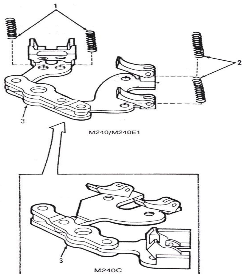
Pawl assembly, feed, M240/M240E1 11826177 and M240C 11826017
