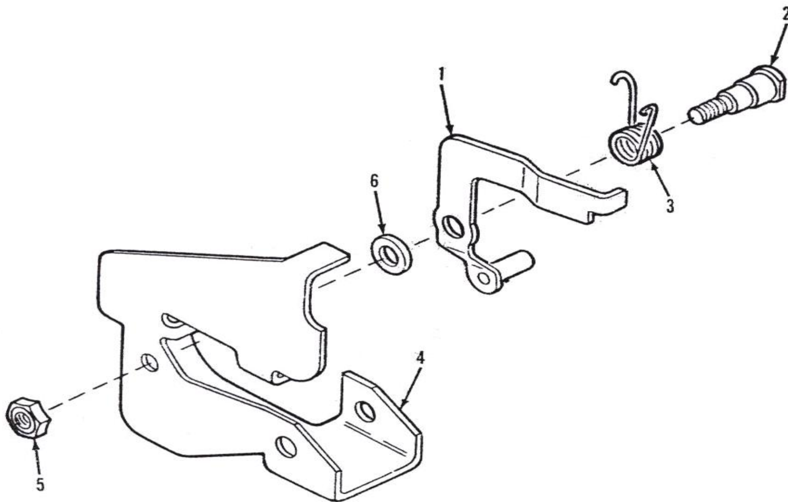
Actuating assembly, trigger, M240E1, 12597071
