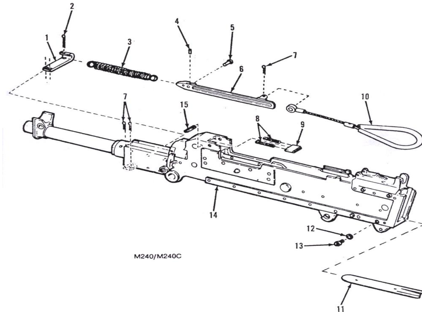
Receiver assembly, M240/M240C, 11826192 and M240E1 12597044 (Sheet 1 of 2)
