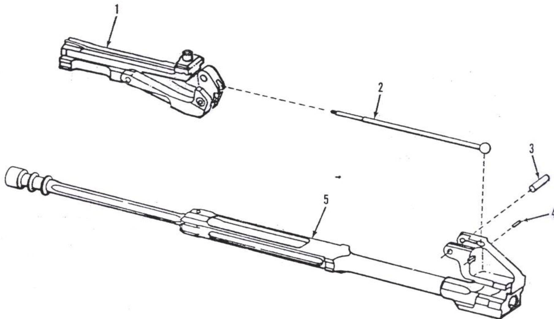
Bolt and operating rod assembly 11826070
