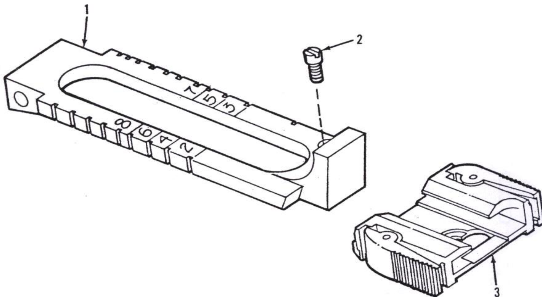
Rear sight assembly, M240E1 12597046
