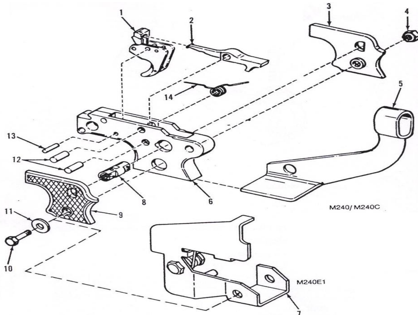
Trigger housing assembly M240/M240C 11826230 and M240E1 12597070
