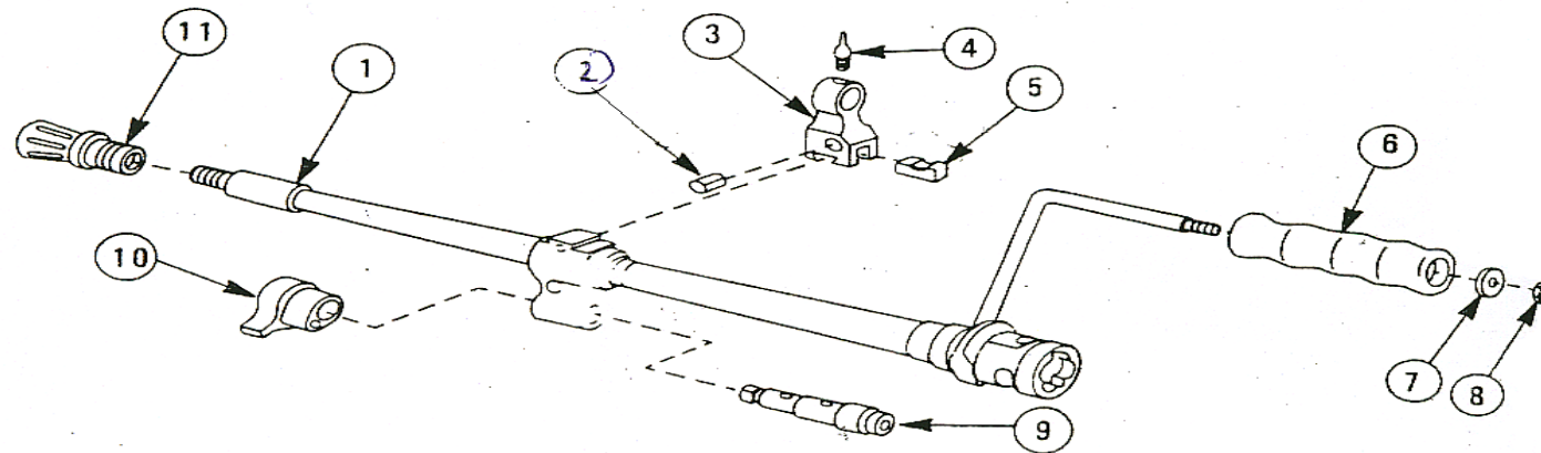
OLD STYLE BARREL ASSEMBLY - 9348420
