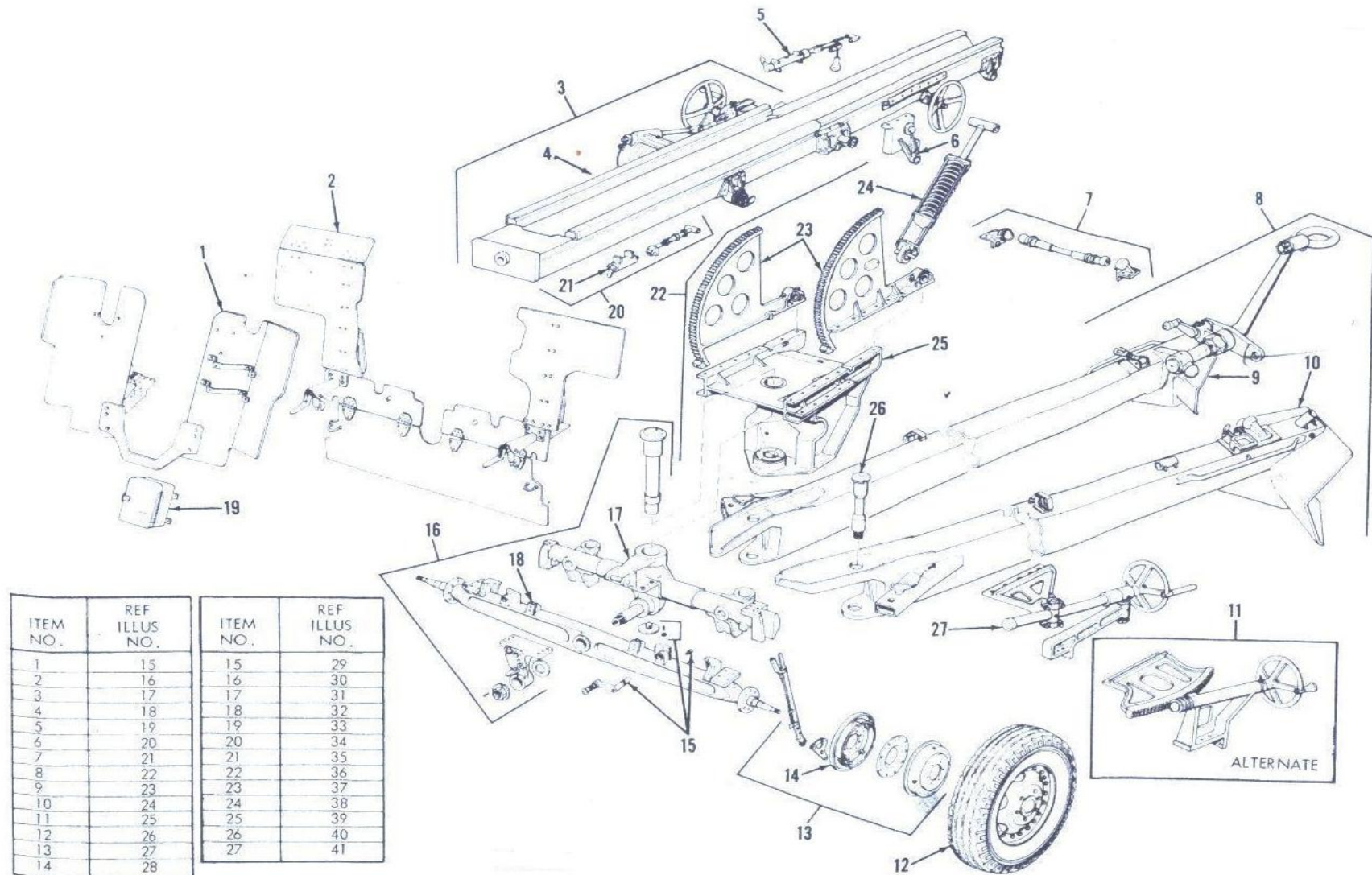
Figure 14. 105-MM howitzer carriage M2A2-partially exploded view.
