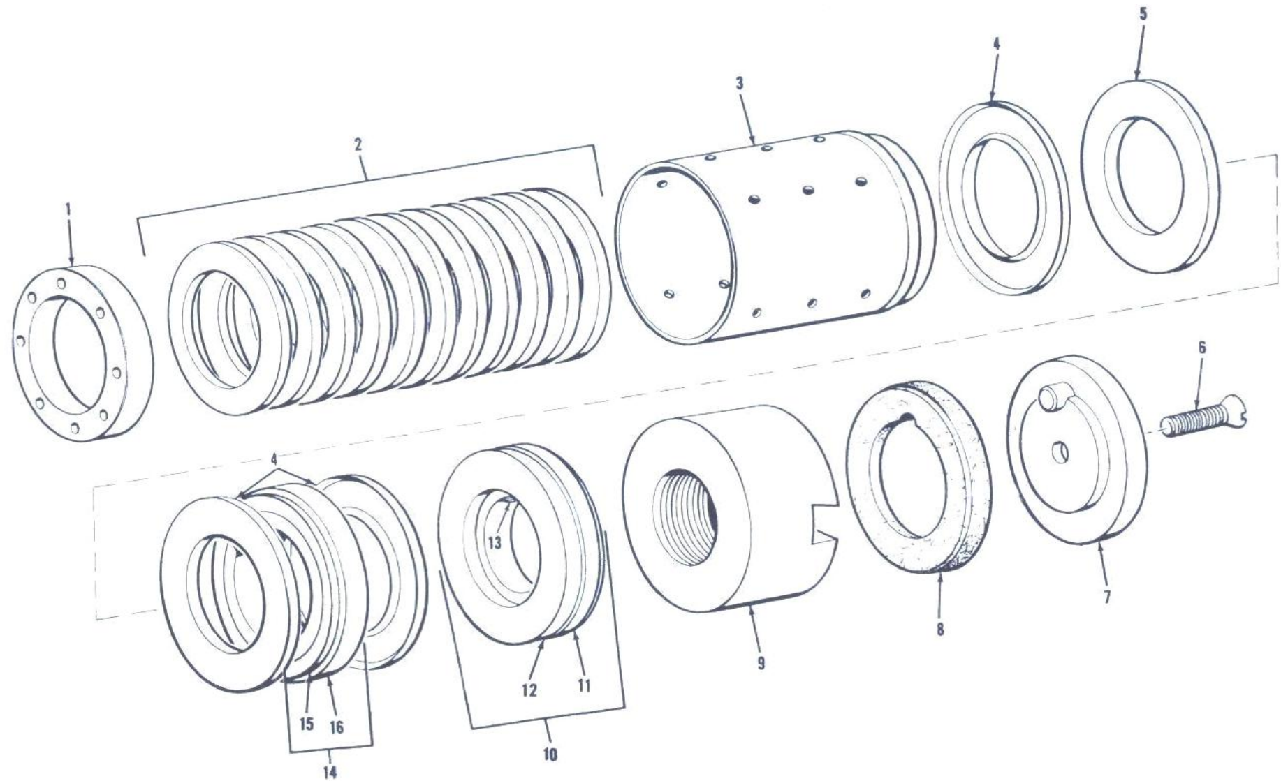
Figure 48. Recoil piston assembly-exploded view.
