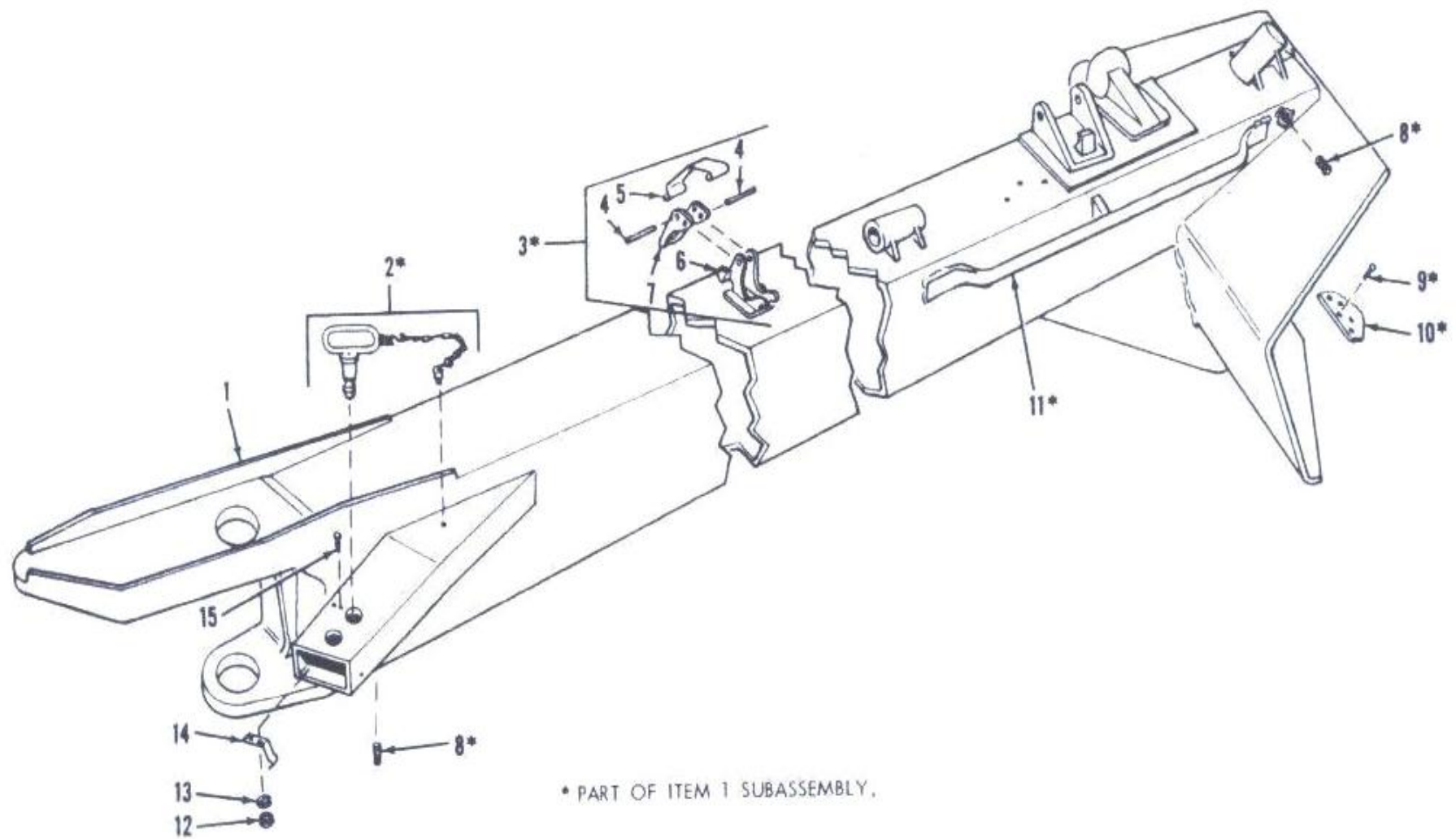
Figure 24. Left trail assembly-exploded view.
