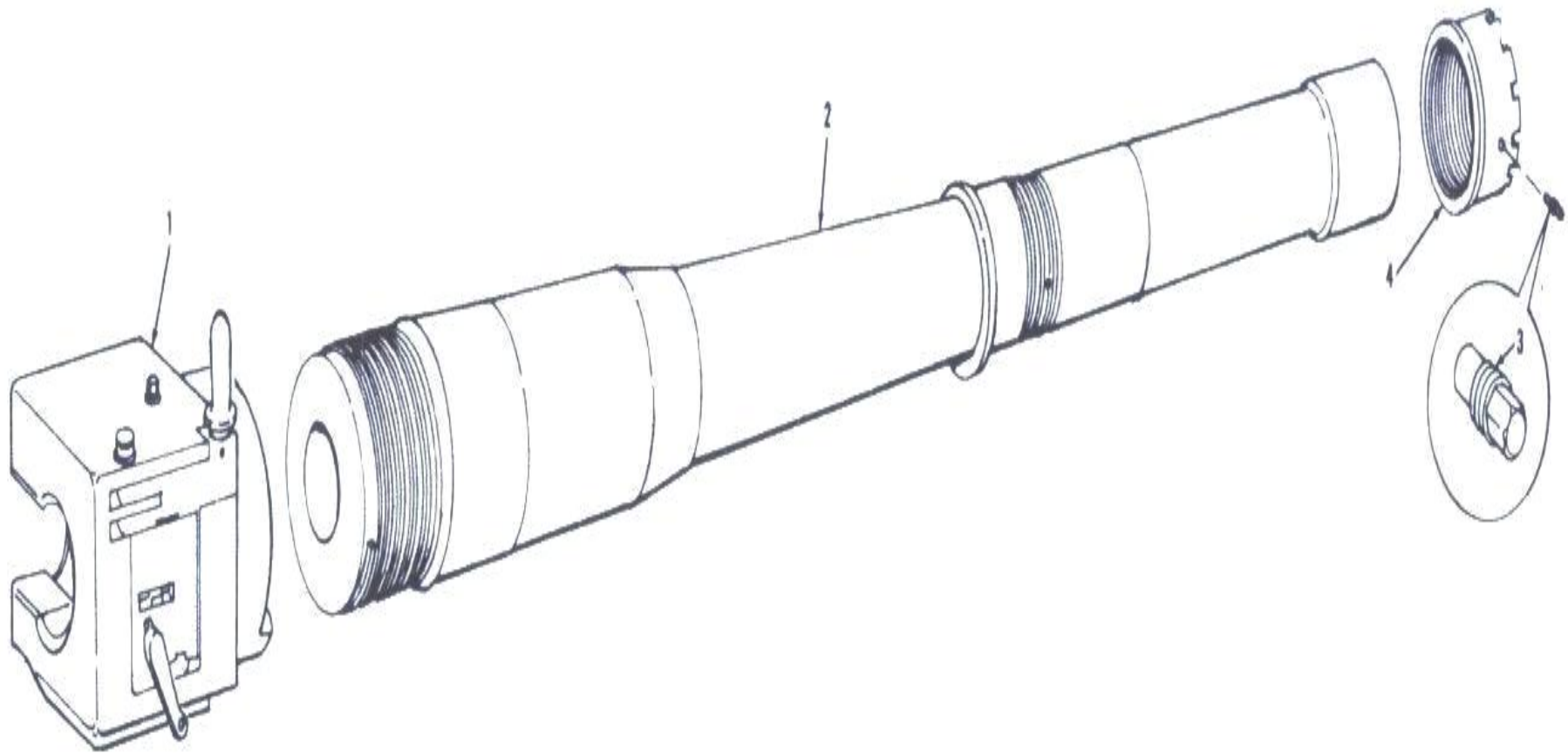
Figure 10. 105-MM howitzer cannon M2A1 and M2A2-partially exploded view.
