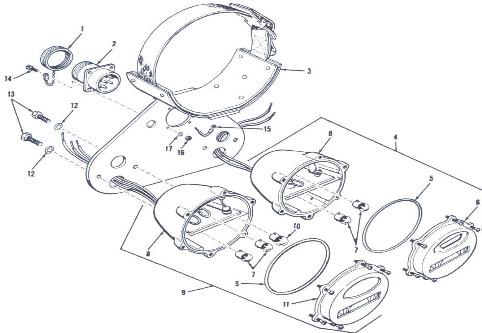
Figure 53. Muzzle bottom tail and stop blackout light-exploded view.
