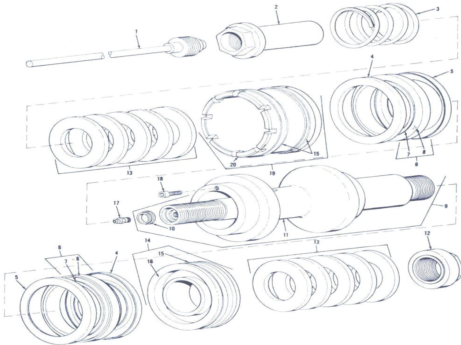
Figure 45. Floating piston assembly-exploded view.
