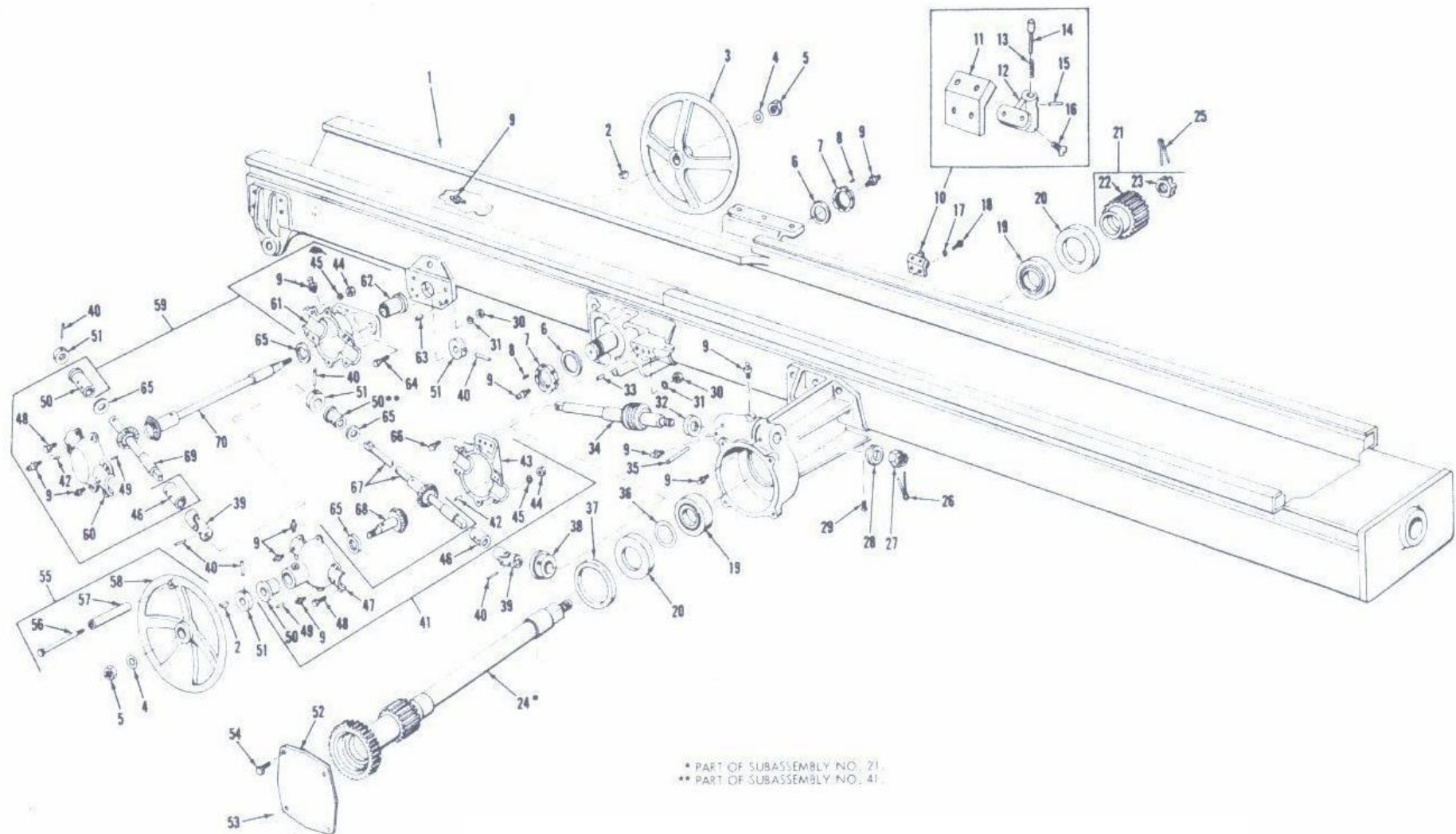
Figure 17. Elevating mechanism assembly-partially exploded view.
