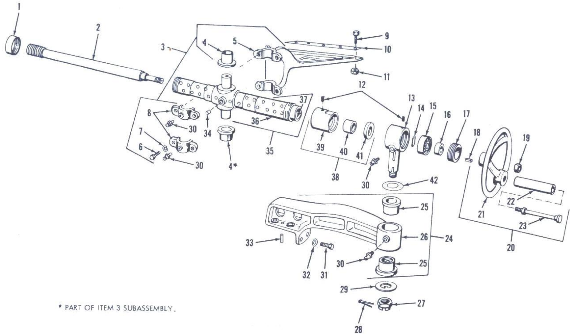
Figure 41. Traversing mechanism assembly-exploded view.
