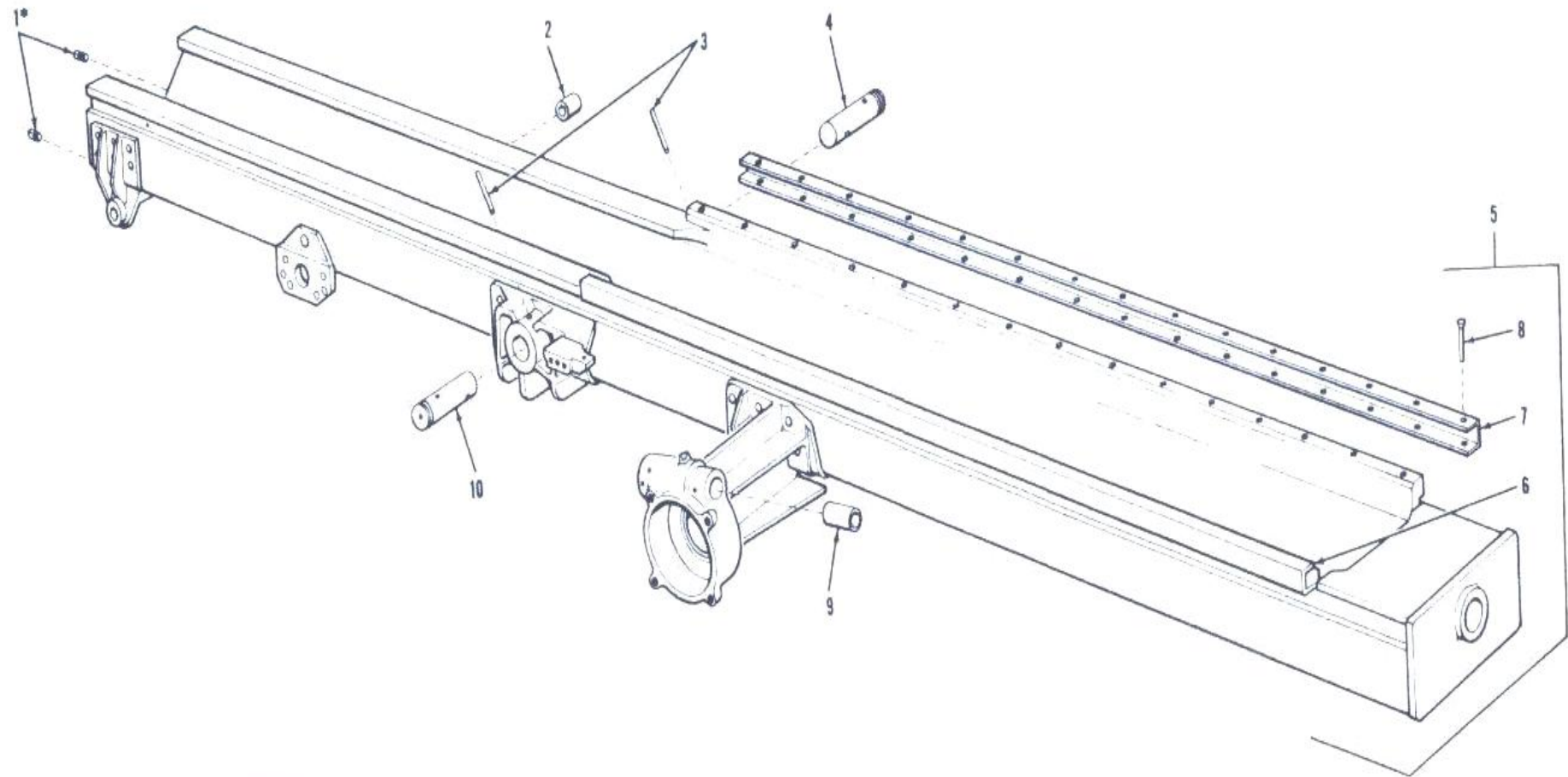
Figure 18. 105-MM howitzer carriage cradle-exploded view.
