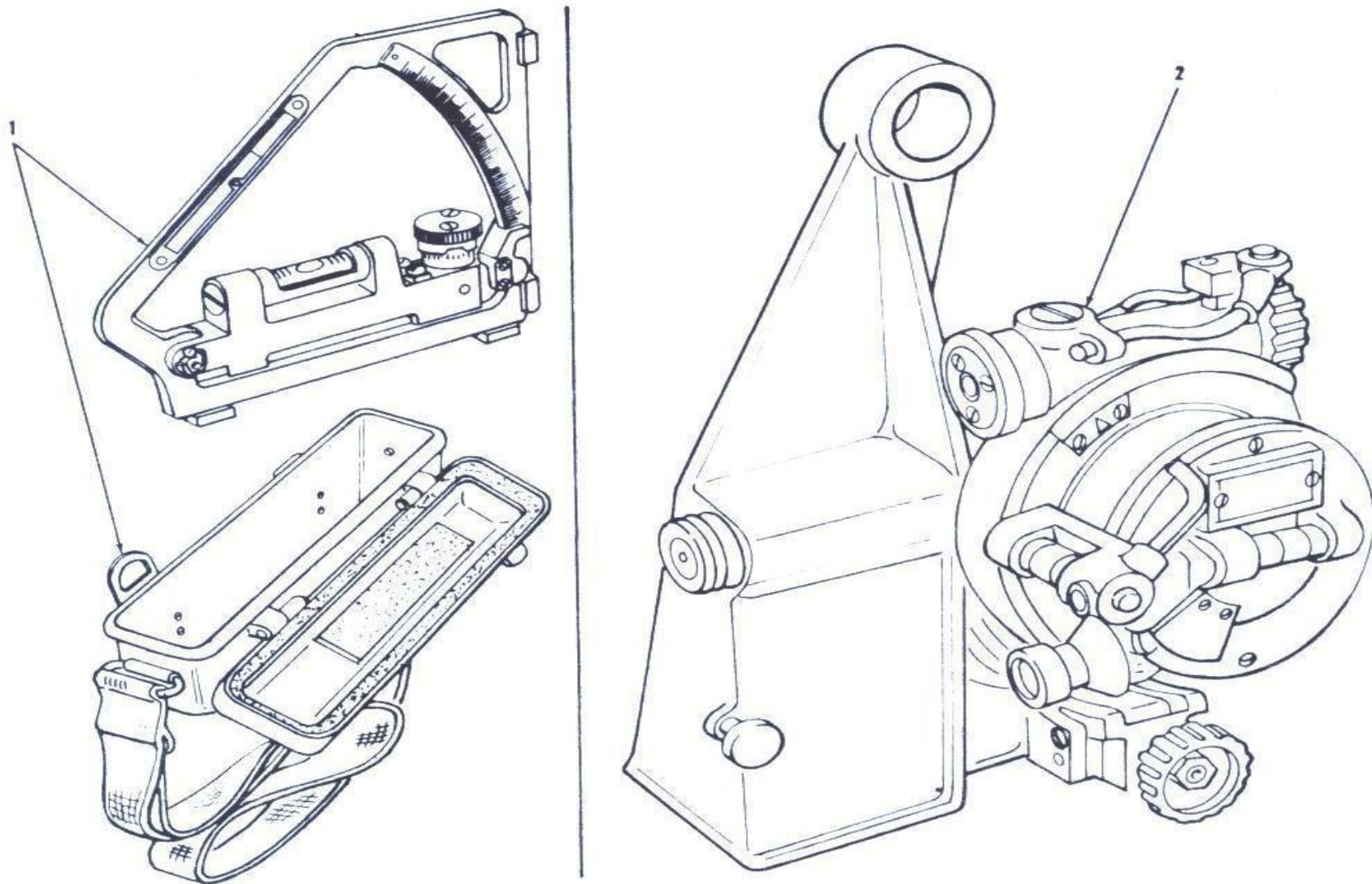
Figure 8. Fire control quadrant M1A1 w/carrying case, and fire control quadrant M4A1.
