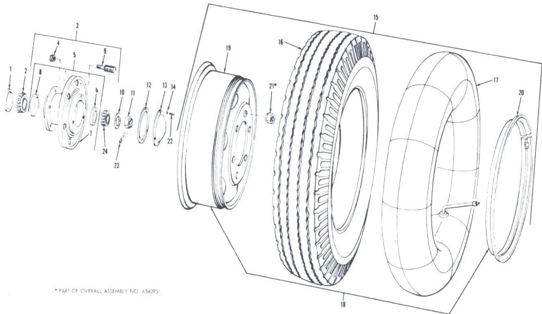
Figure 26. Wheel and hub assembly-exploded view.
