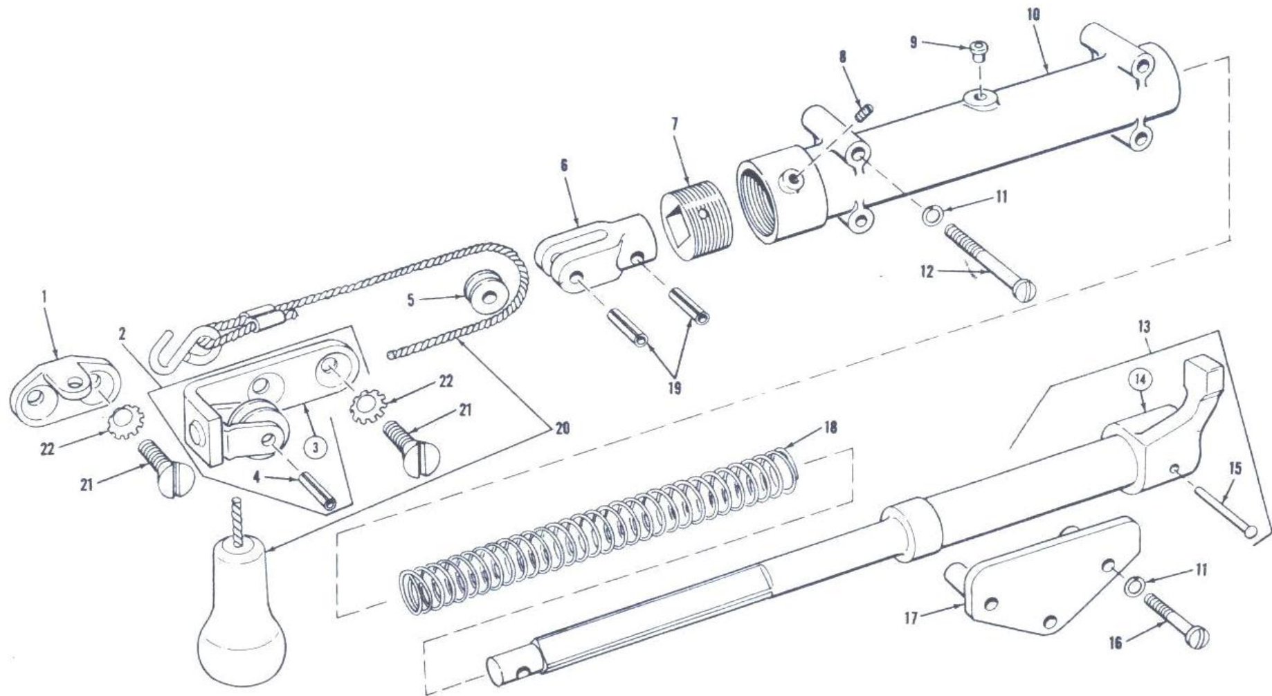
Figure 19. Firing mechanism assembly-exploded view.
