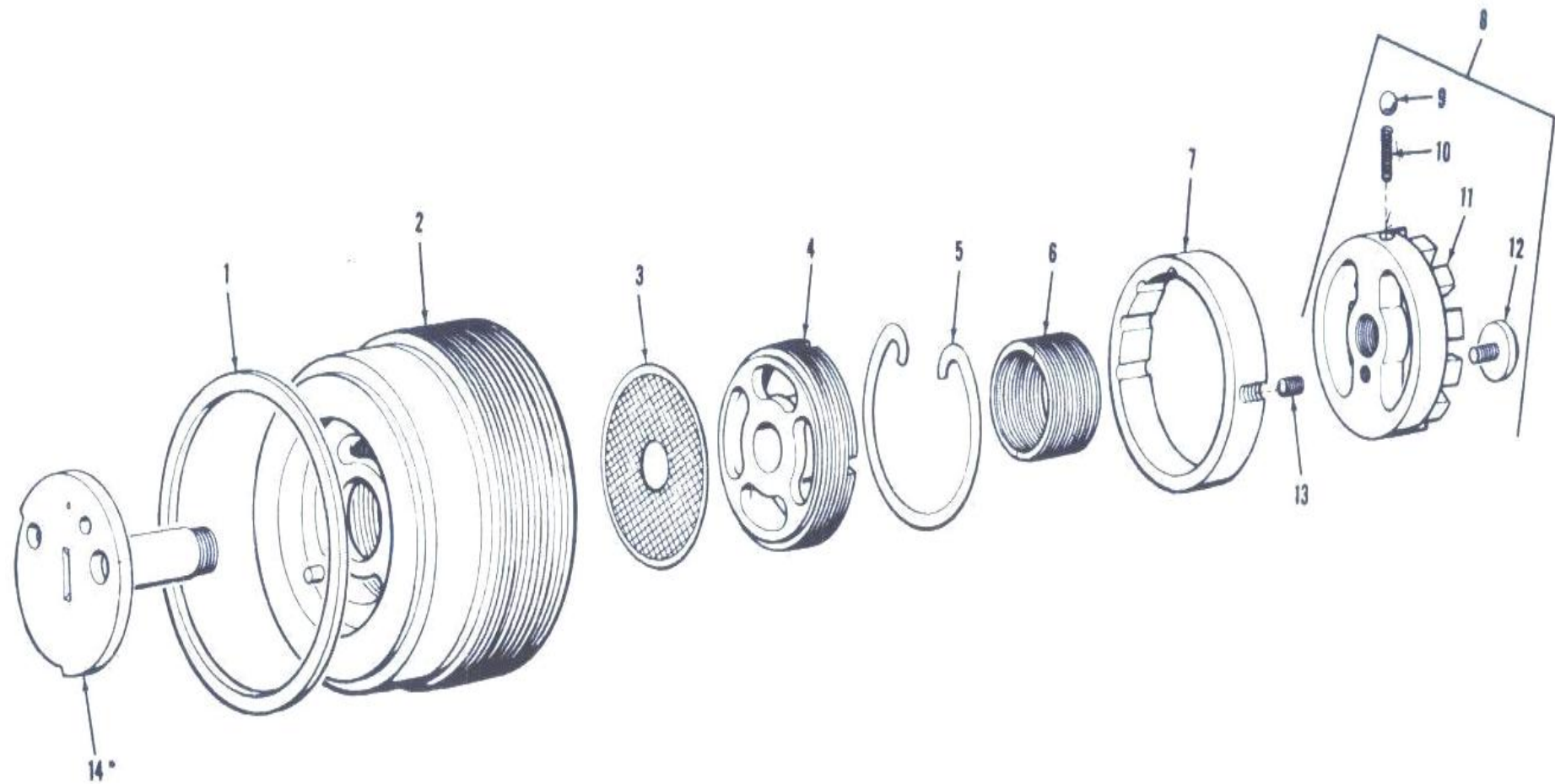
Figure 47. Recoil cylinder respirator assembly-exploded view.
