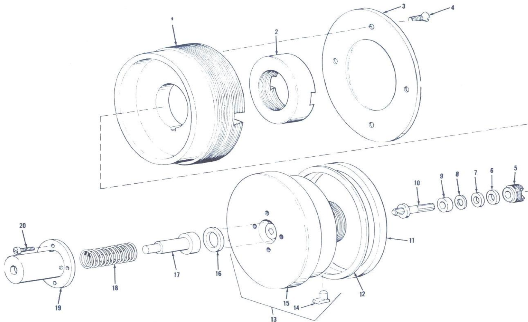
Figure 46. Recuperator cylinder rear head assembly-exploded view.
