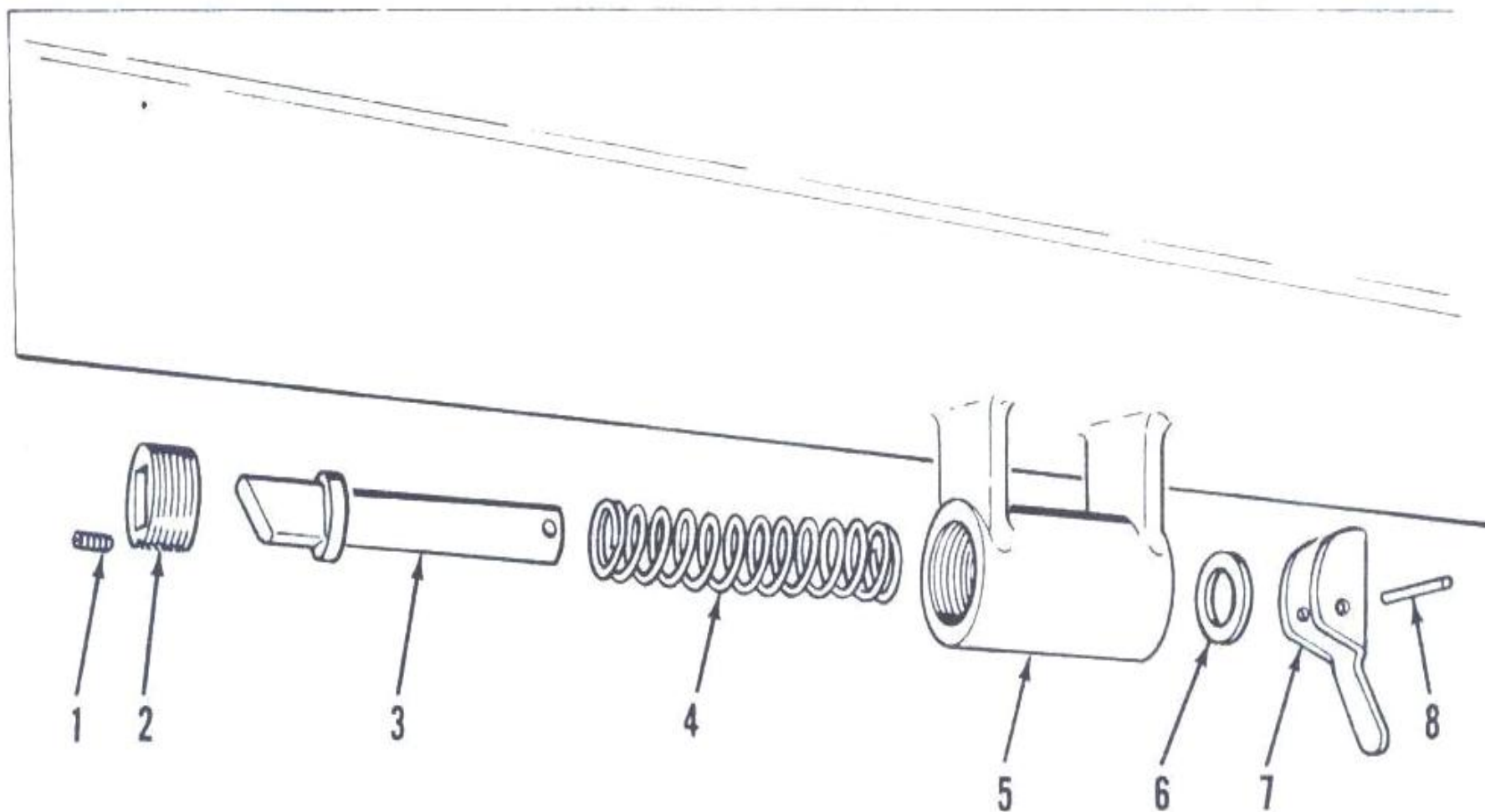
Figure 35. Strut latch assembly-exploded view.
