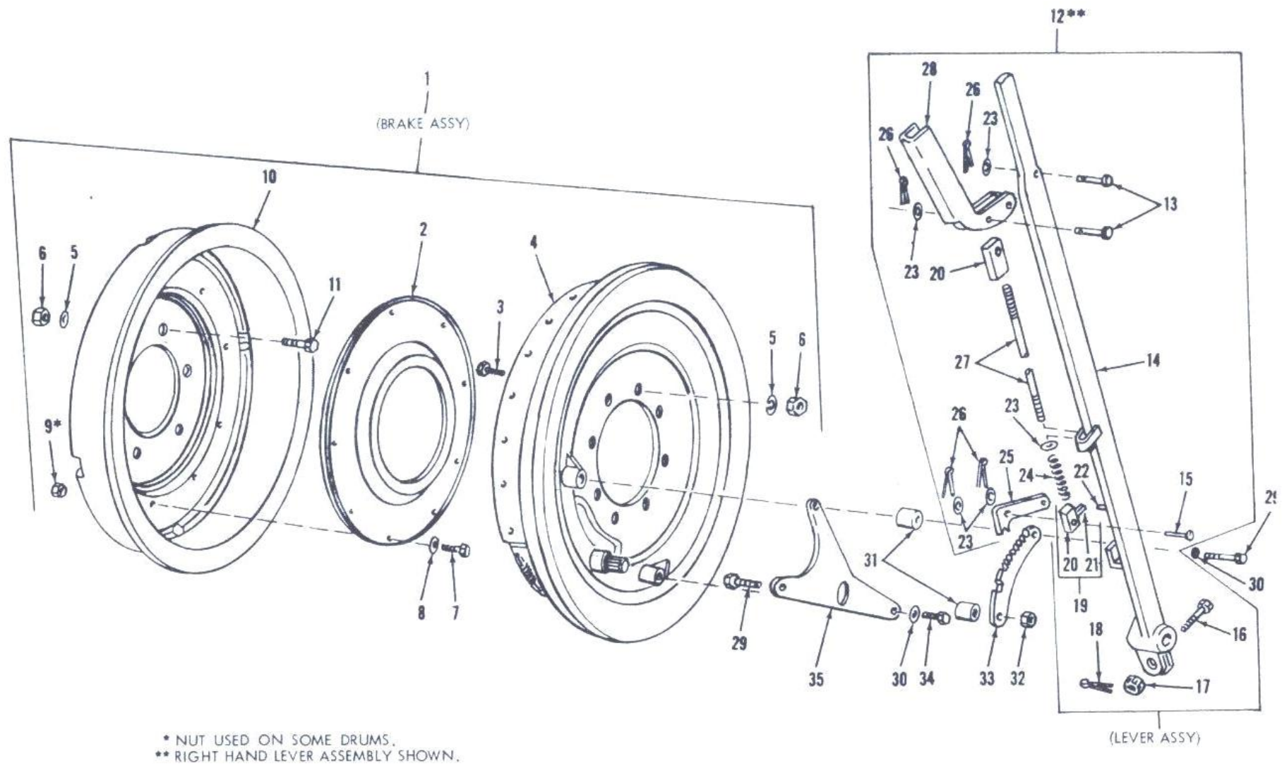
Figure 27. Brake operating mechanism assembly-partially exploded view.
