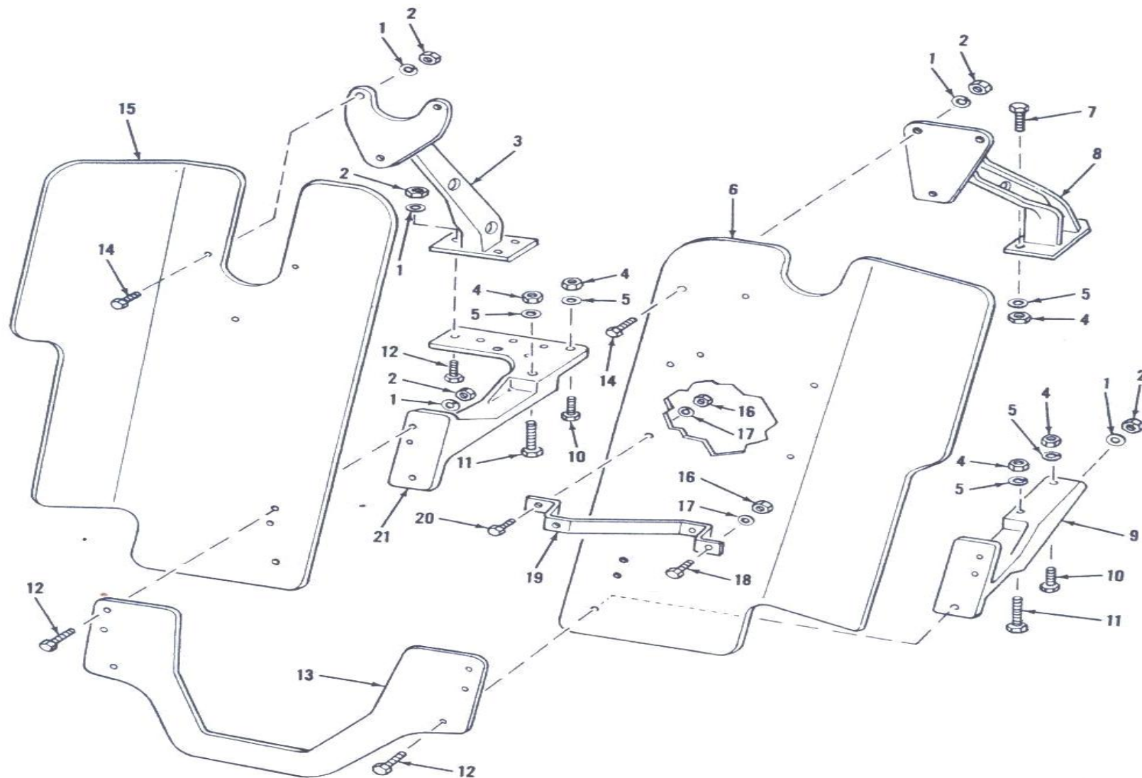
Figure 15. Auxiliary shield assembly-exploded view.
