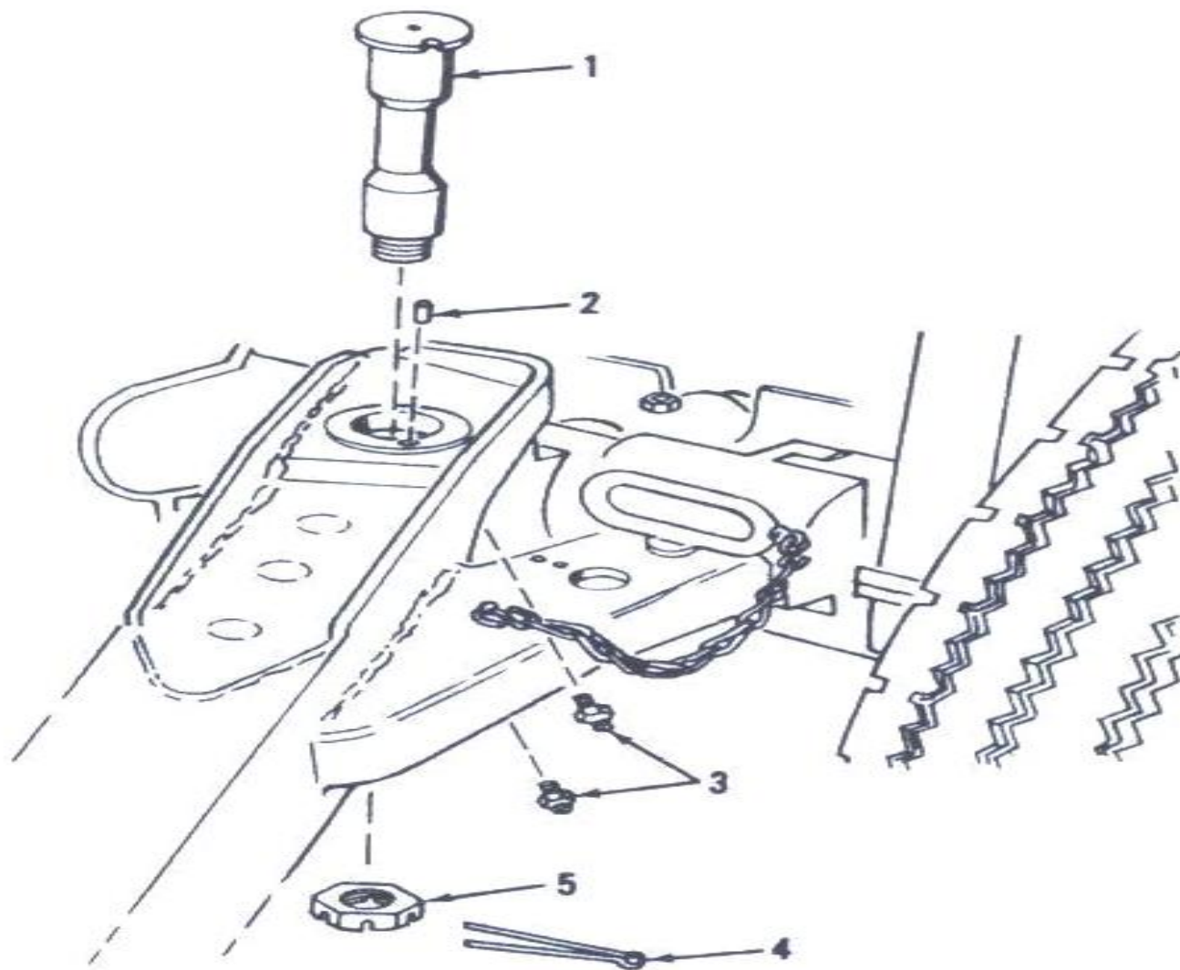
Figure 40. Trail hinge pin assembly-exploded view.
