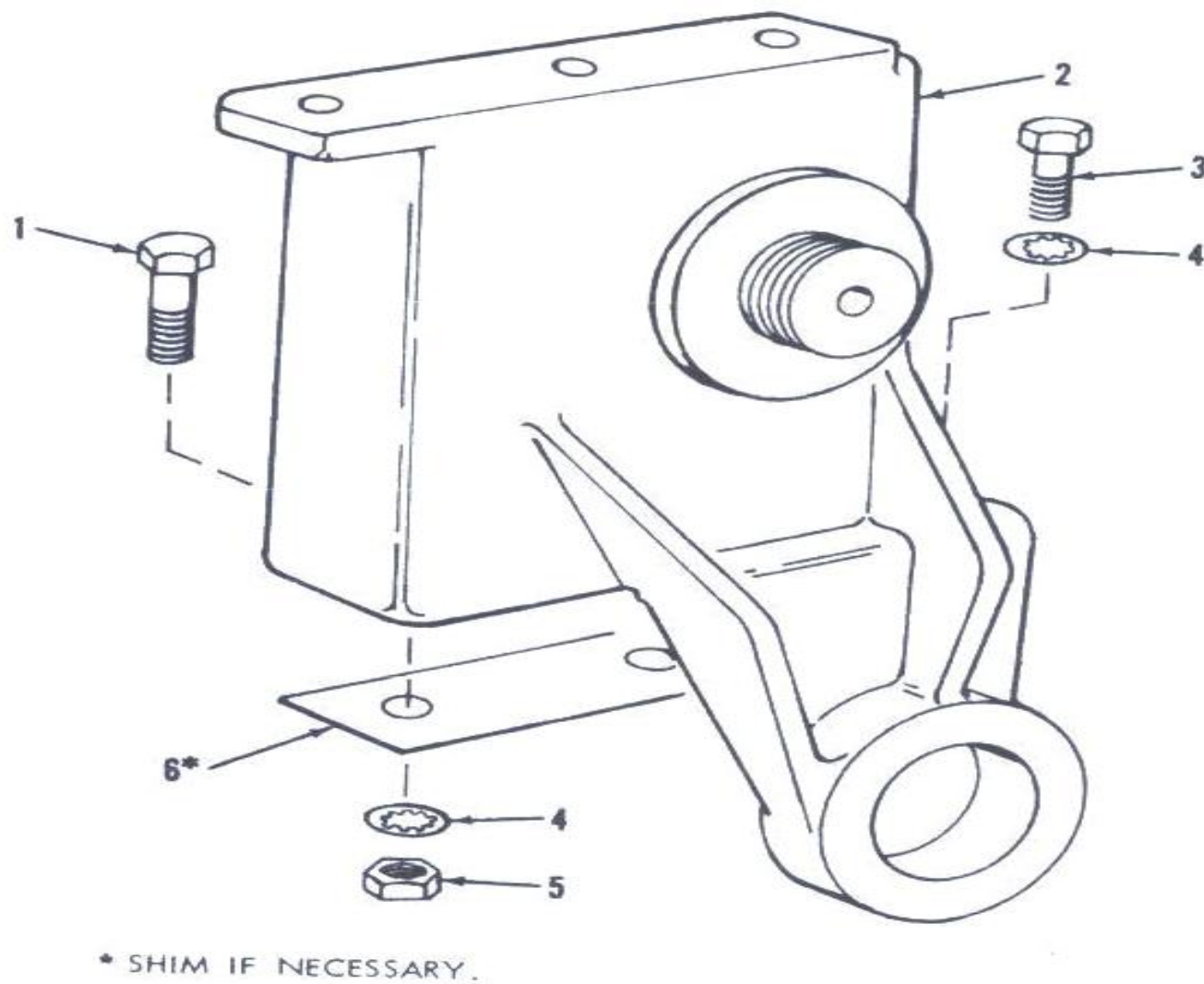
Figure 20. Sight bracket assembly-exploded view.
