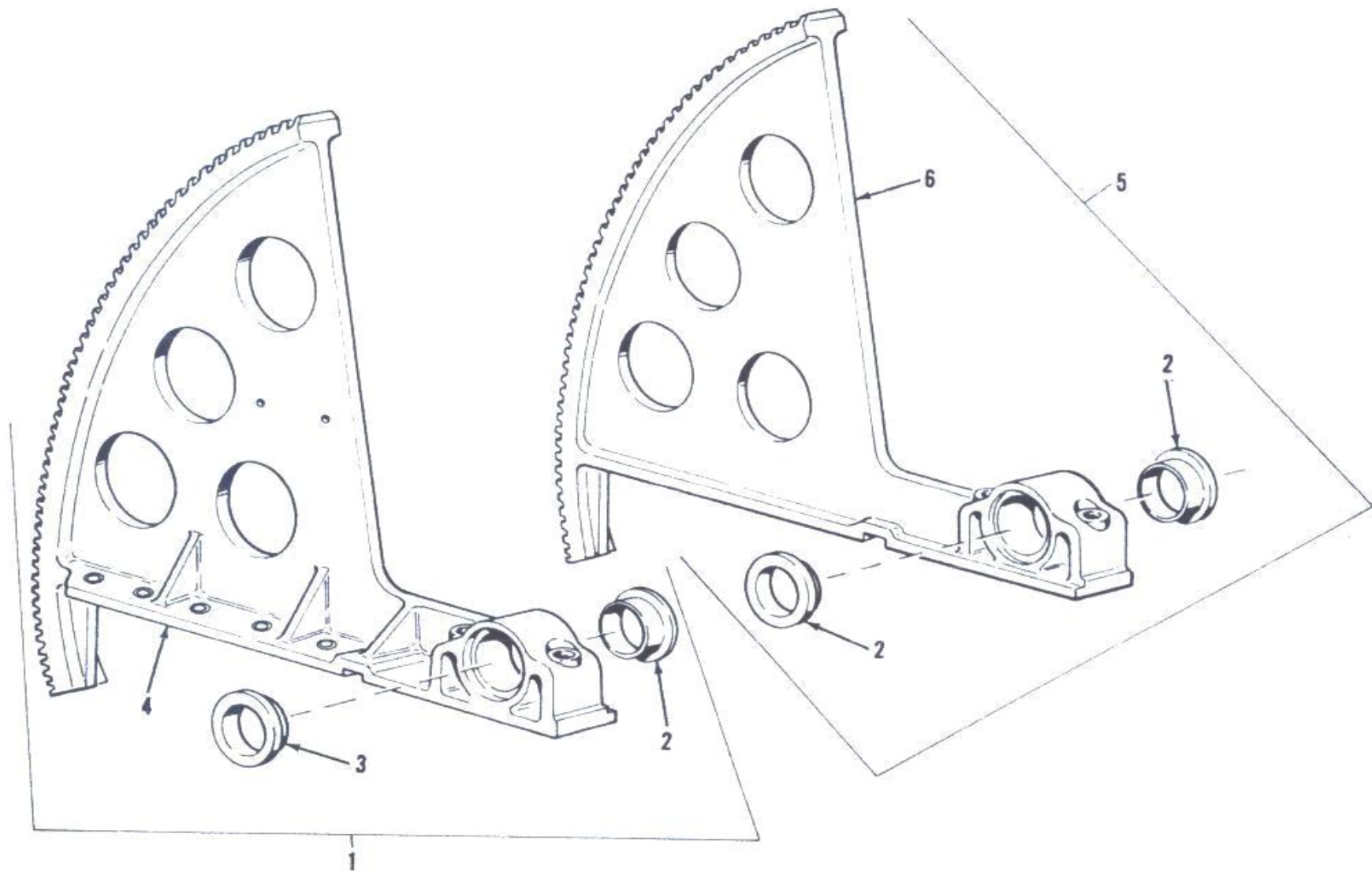
Figure 37. Left and right elevating arc assembly-exploded view.
