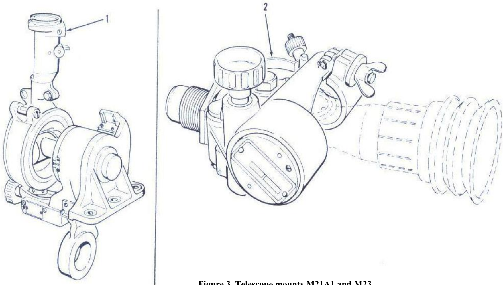
Figure 3. Telescope mounts M21A1 and M23.
