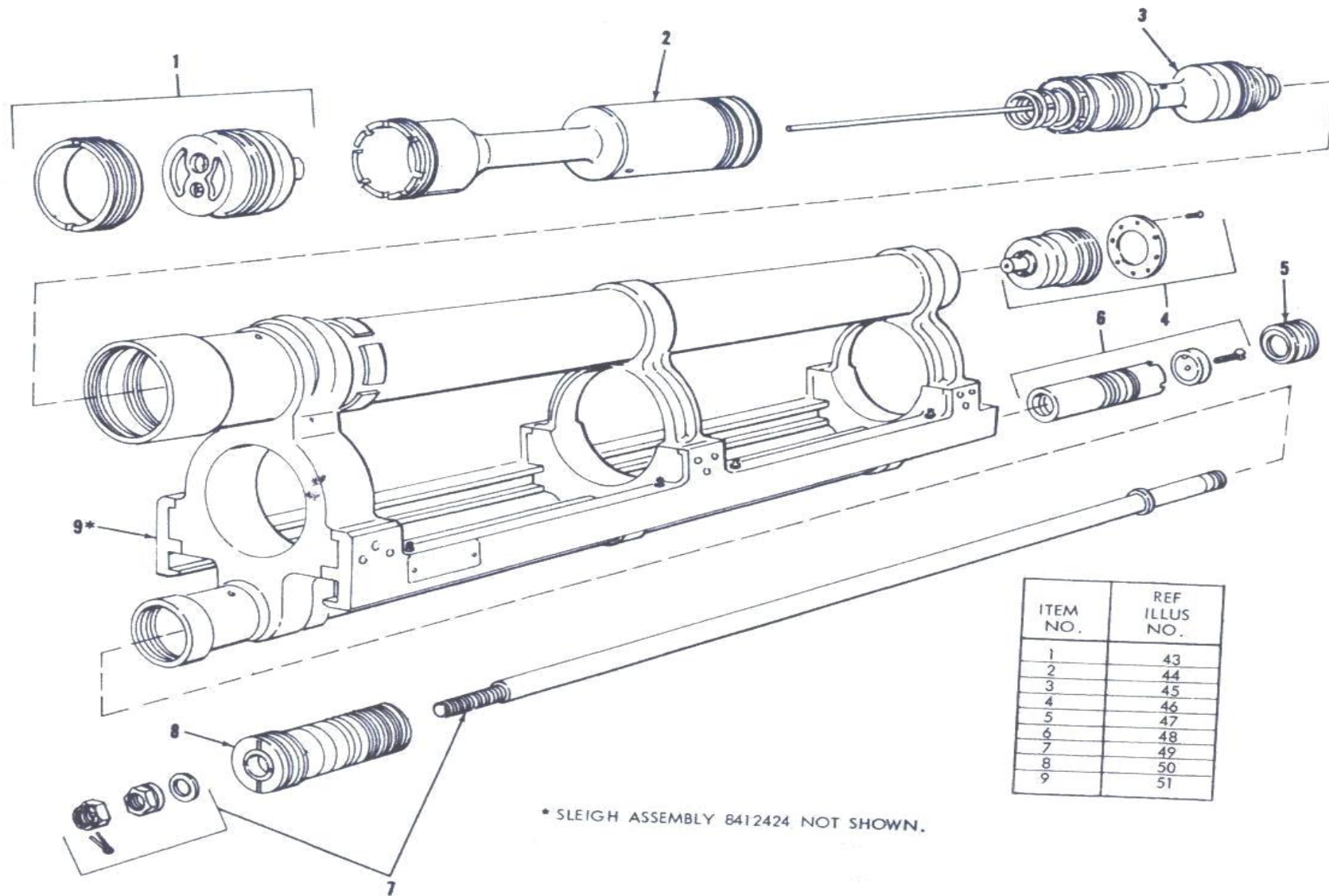
Figure 42. 105-MM howitzer recoil mechanism M2A4 and M2A5-partially exploded view.
