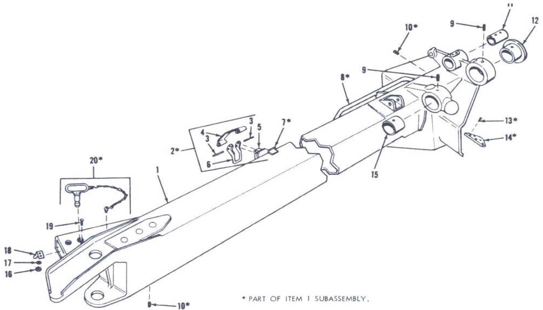
Figure 23. Right trail assembly-exploded view.
