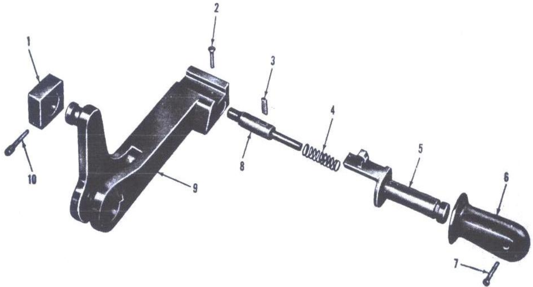
Figure 12. Breechblock operating lever-exploded view.
