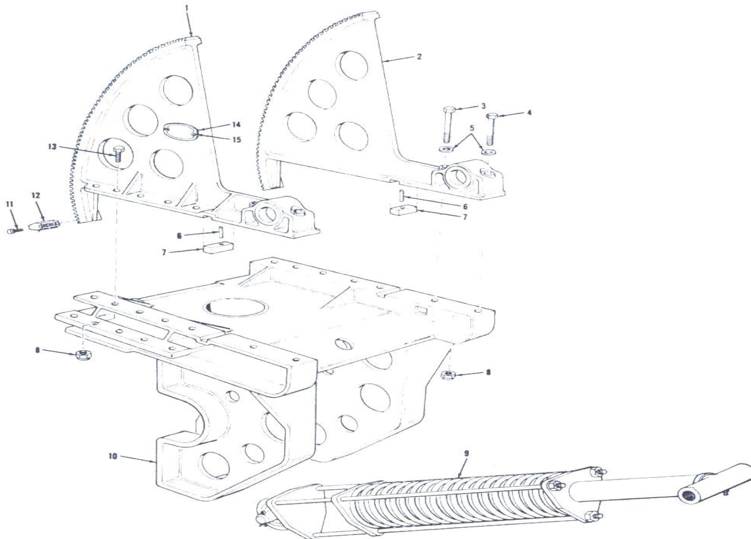
Figure 36. Top carriage, elevating arc, and equilibrator assembly-partially exploded view.
