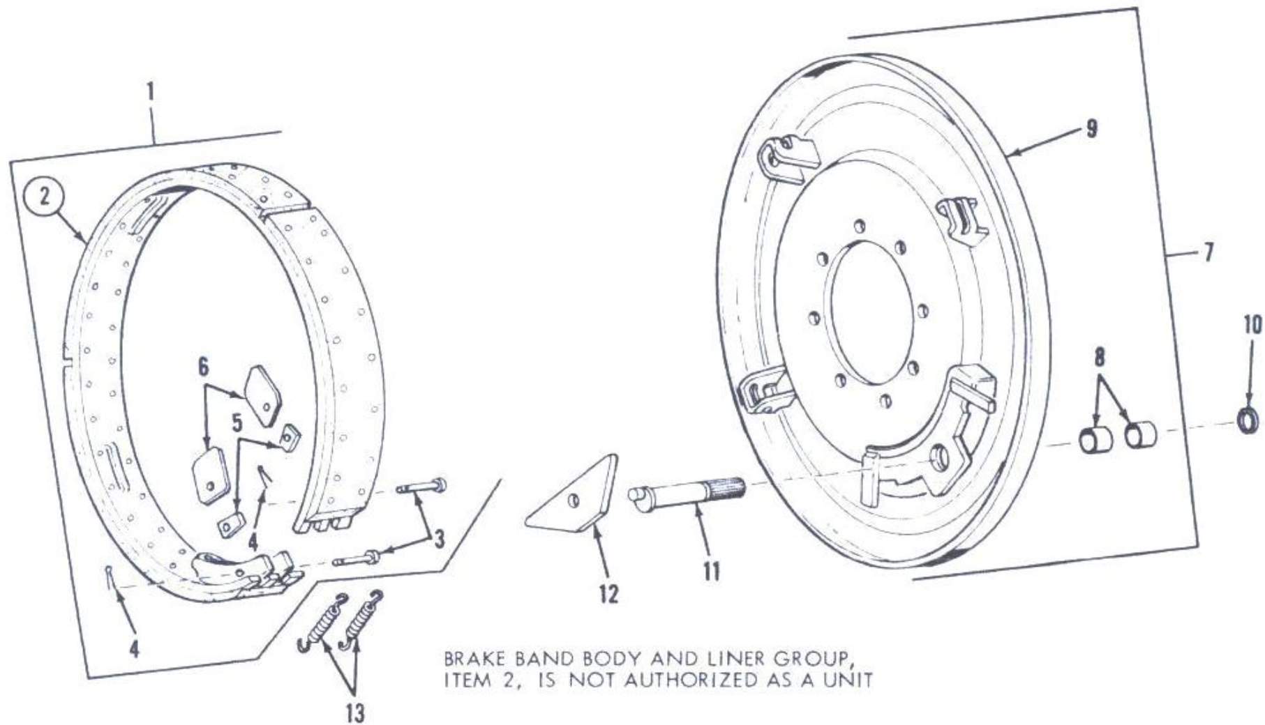
Figure 28. Brake backing plate assembly-exploded view.
