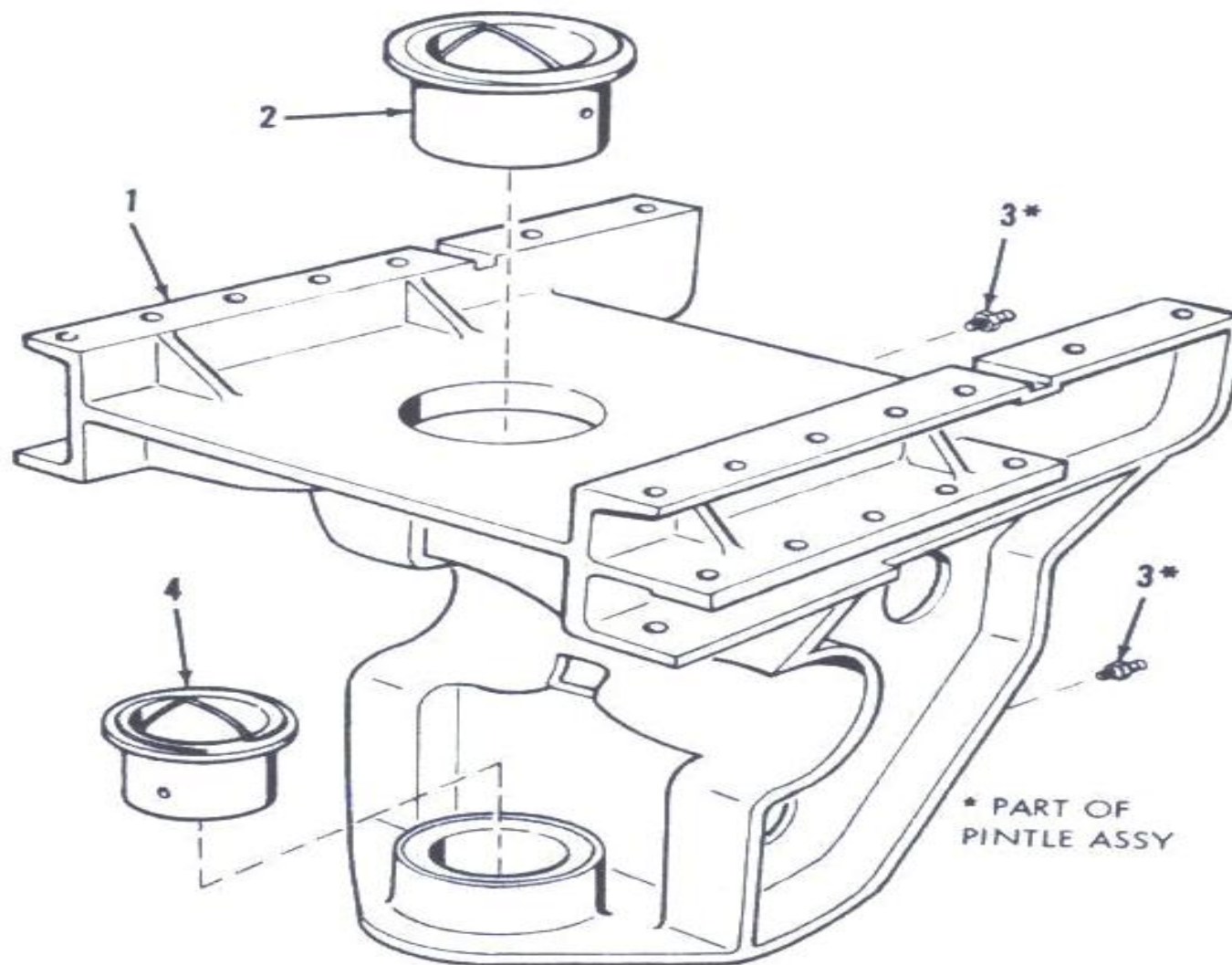
Figure 39. Top carriage assembly-exploded view.
