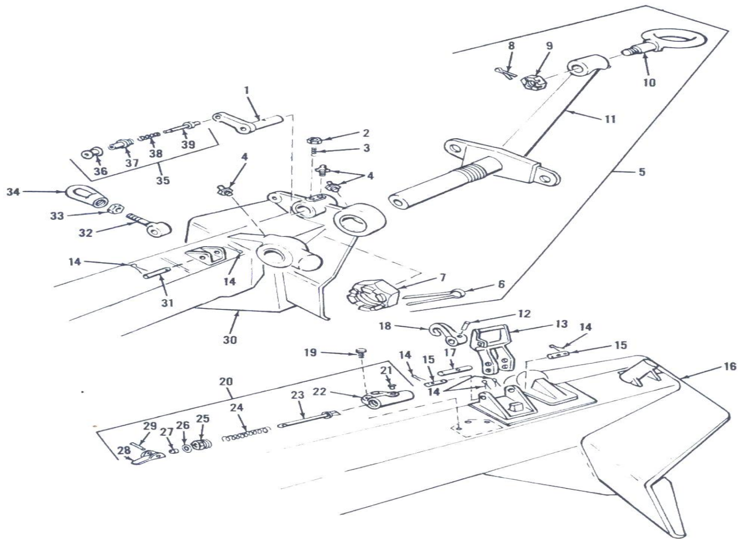
Figure 22. Trail and spade assembly-partially exploded view.
