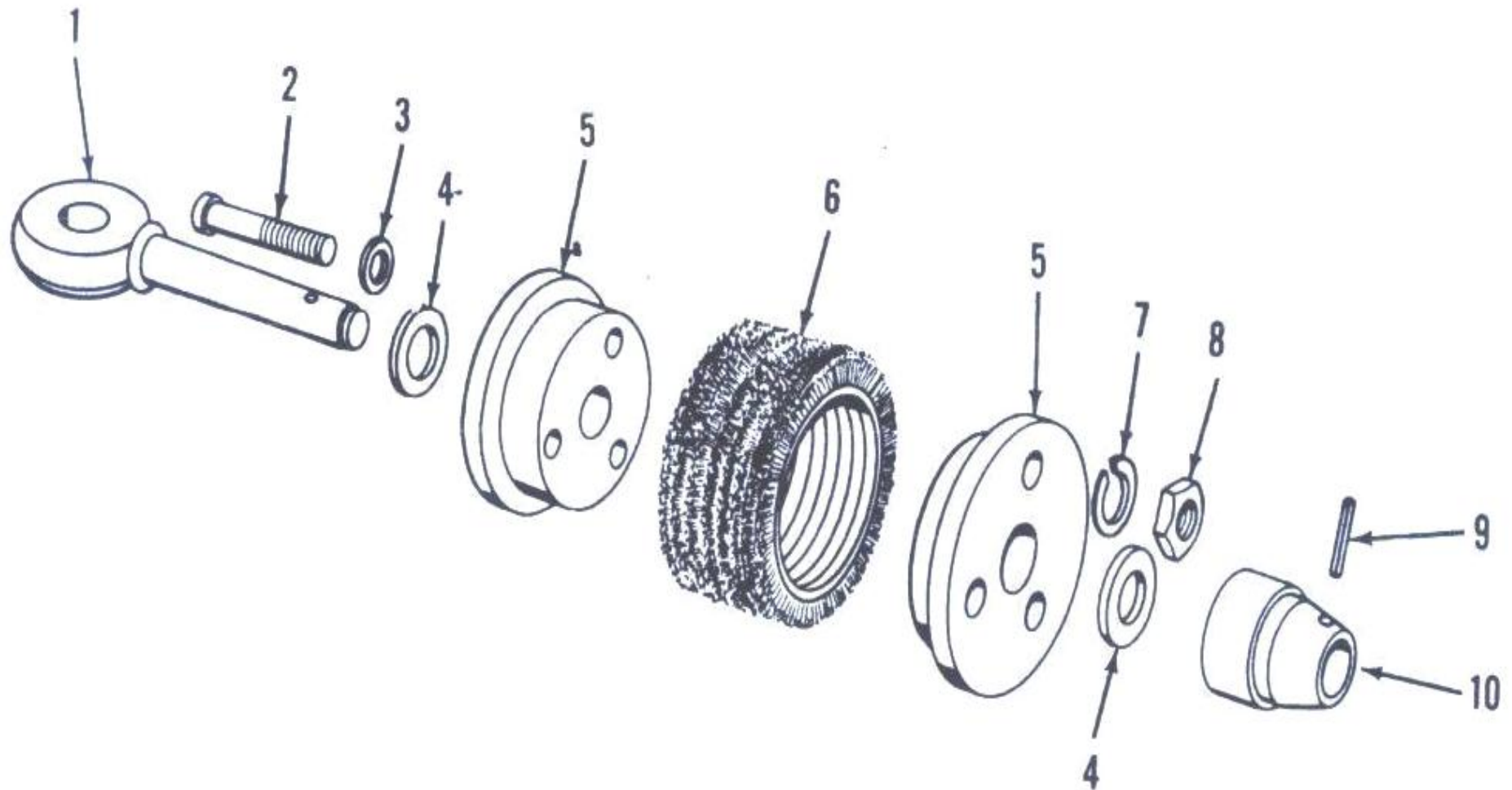
Figure 52. Bore brush-exploded view.
