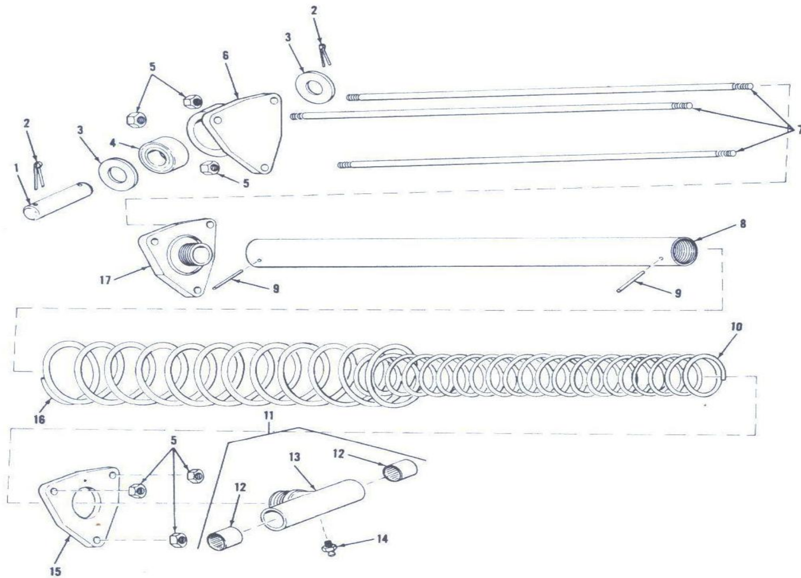
Figure 38. Equilibrator assembly-exploded view.
