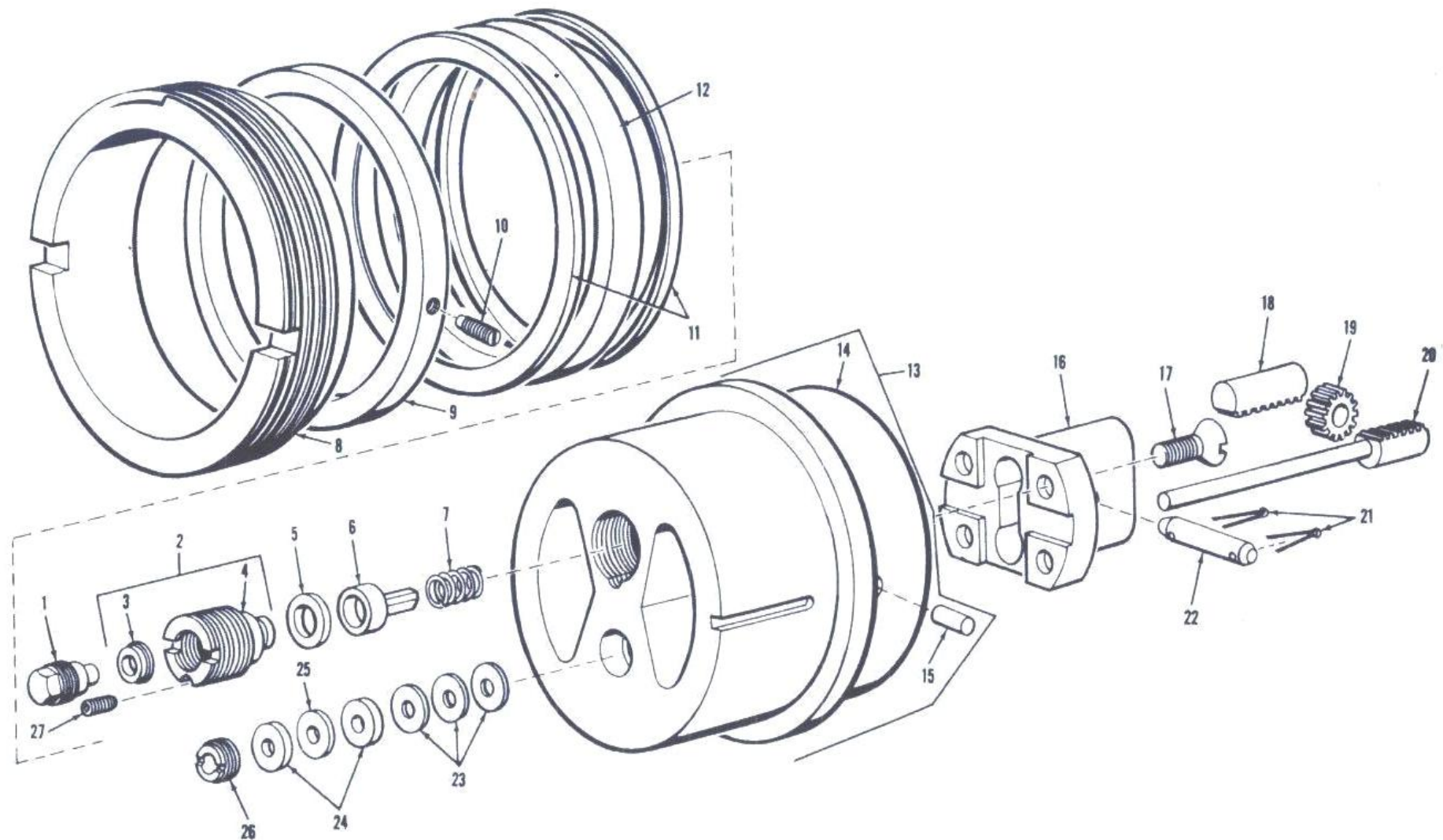
Figure 43. Recuperator cylinder front head assembly-exploded view.
