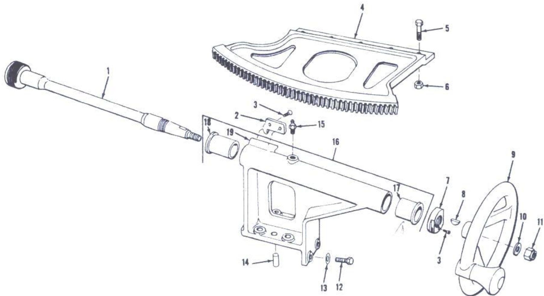
Figure 25. Traversing mechanism assembly-exploded view.
