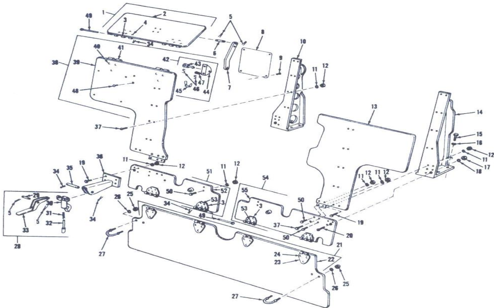
Figure 16. Shield assembly-exploded view.
