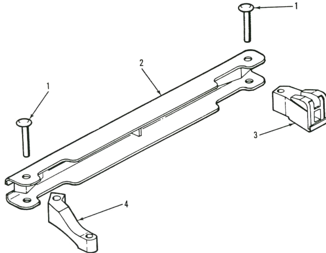
Figure C-9. Sightarm Assembly
