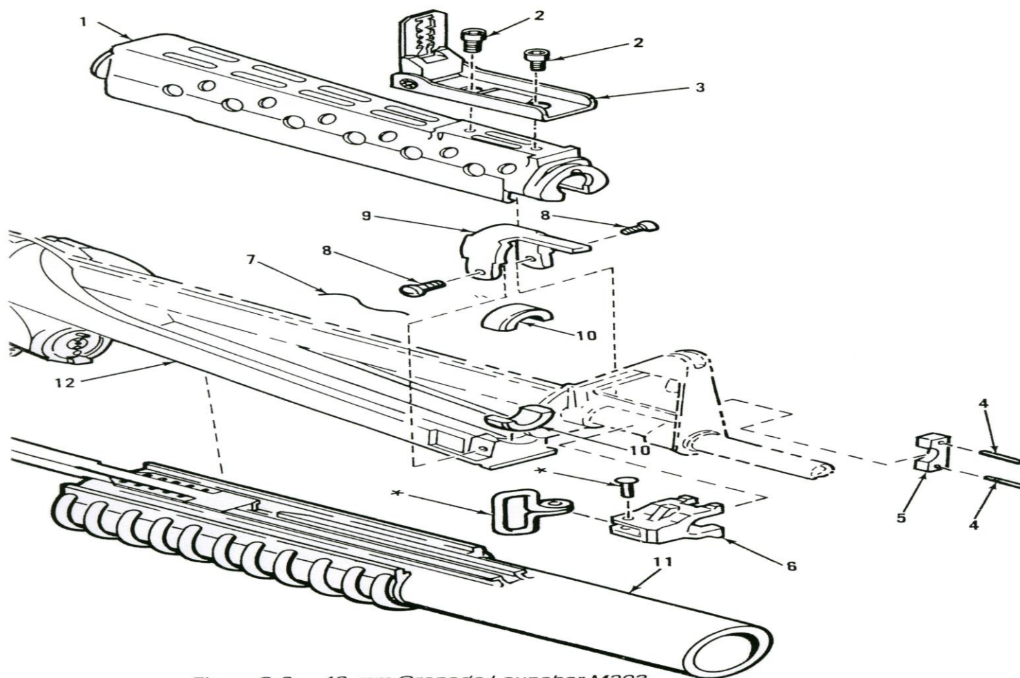
Figure C-2. 40-mm Grenade Launcher M203
