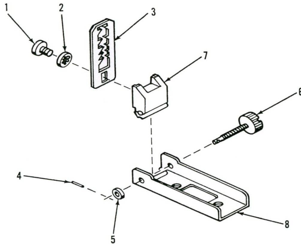
Figure C-3. Leaf Sight Assembly
