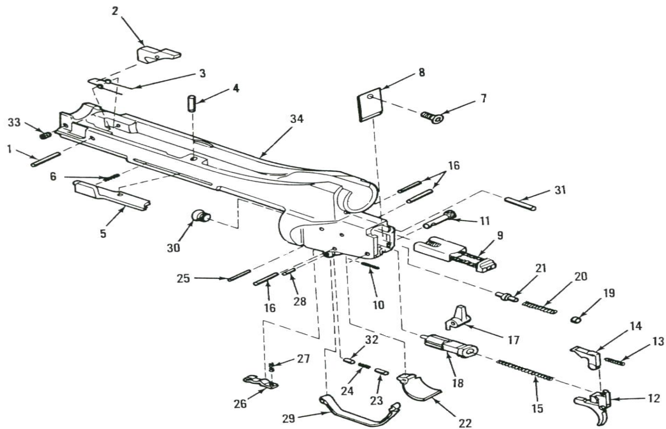
Figure C-5. Receiver Assembly
