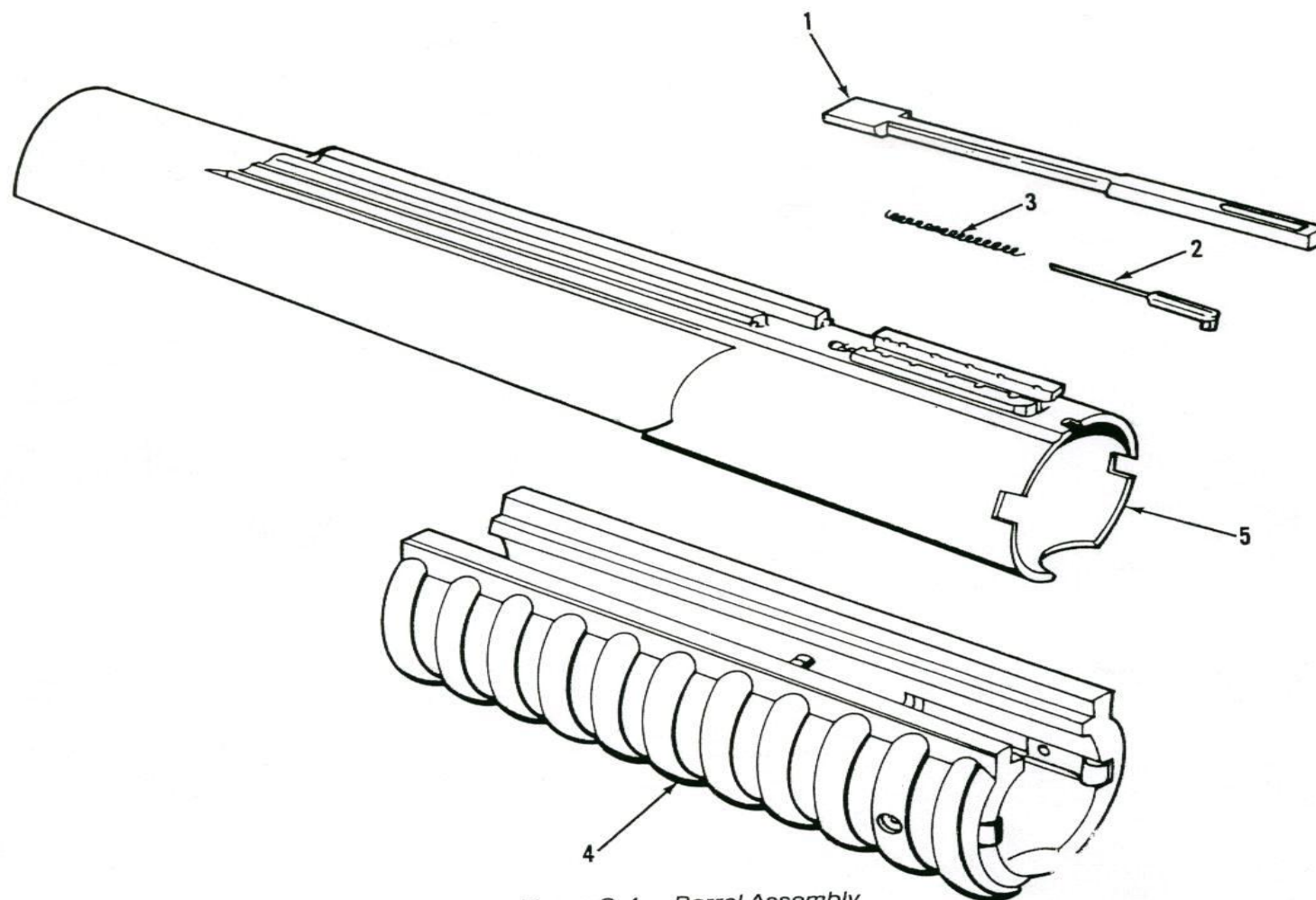
Figure C-4. Barrel Assembly
