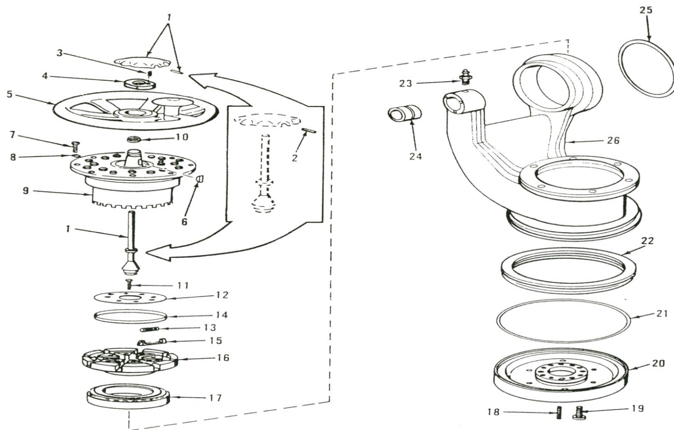
Figure 23. Traversing assembly and shaft assembly.
