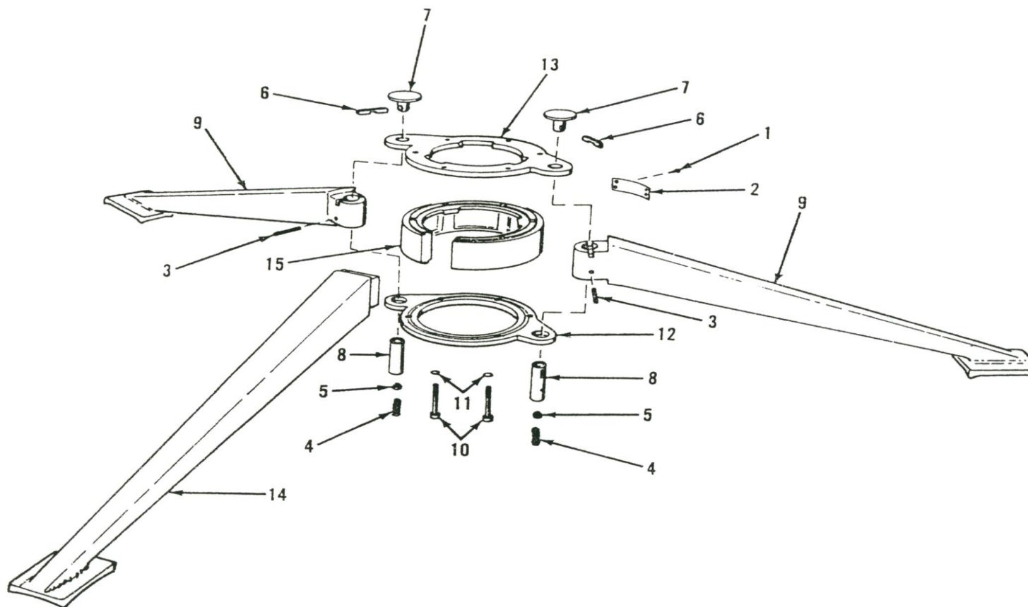
Figure 29. Tripod, rifle mount: M27.
