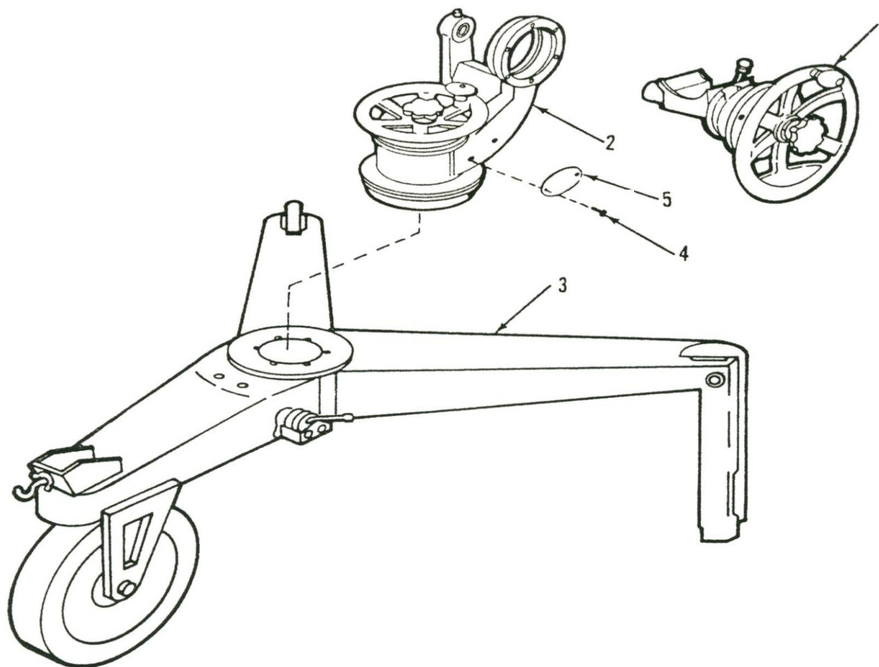
Figure 19. Mount, rifle, 106-mm: M79.
