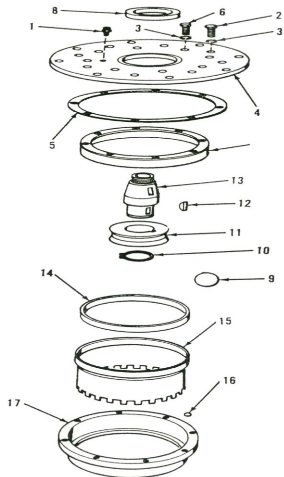
Figure 24. Traversing drive assembly.
