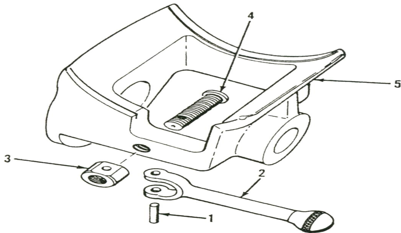
Figure 22. Elevating cradle assembly.
