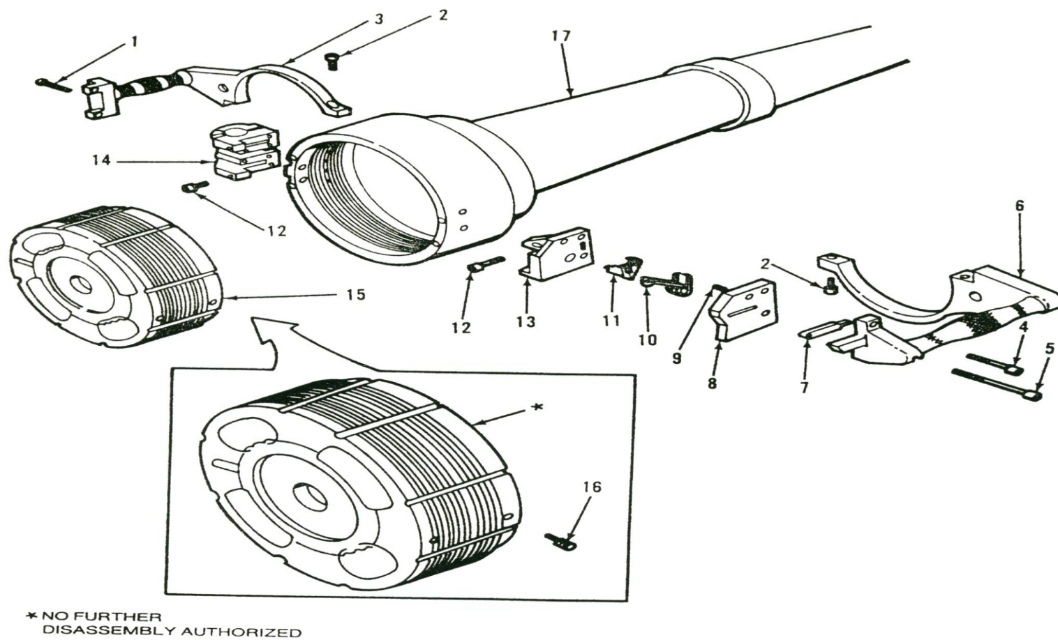
Figure 13. Cannon, 106-mm: M206 and vent assembly.
