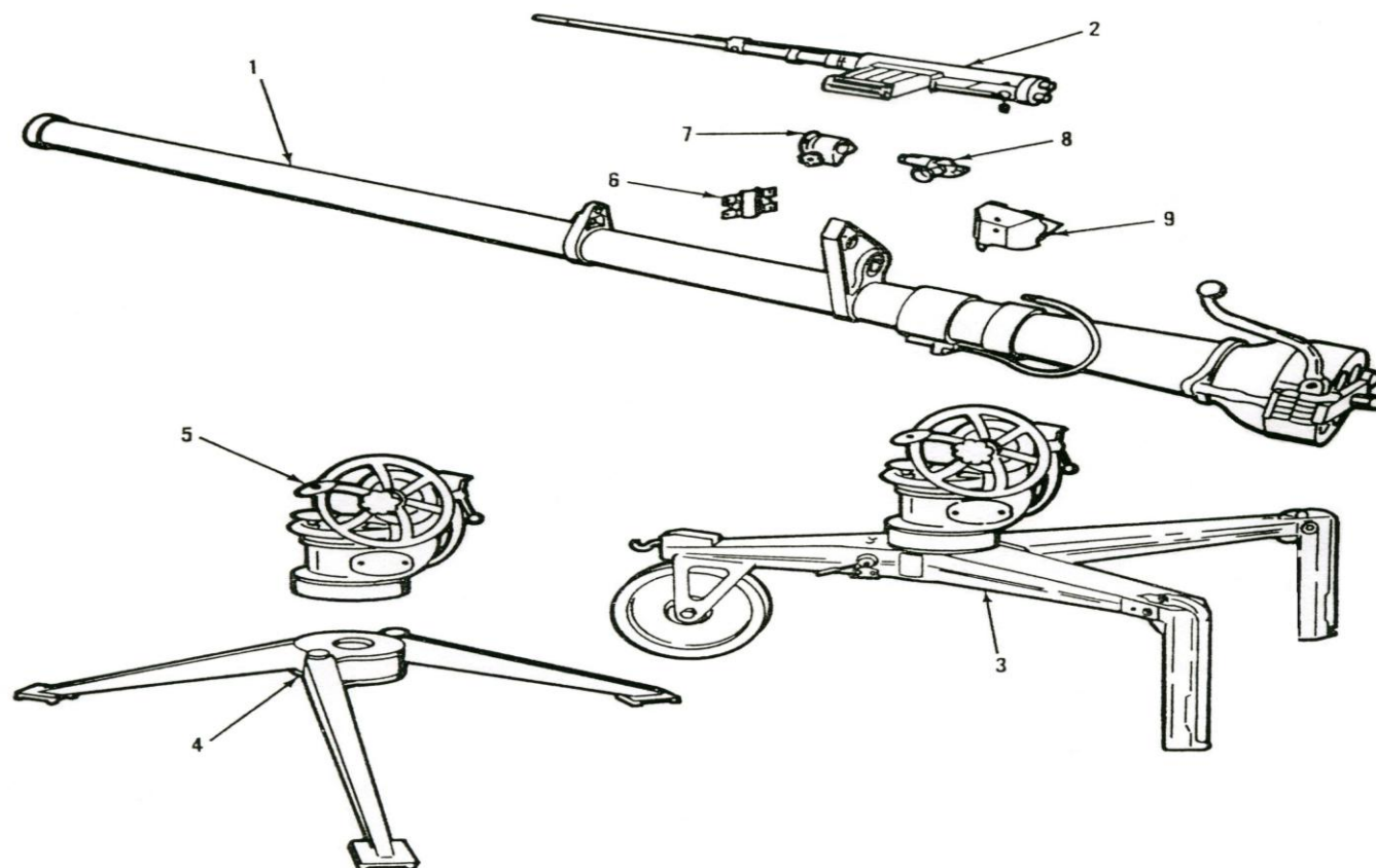
Figure 1. Rifle, recoilless, 106-mm: M40A2 or M40A4.
