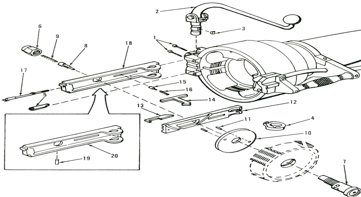
Figure 12. Cannon, 106-mm: M206 and hinge assembly.
