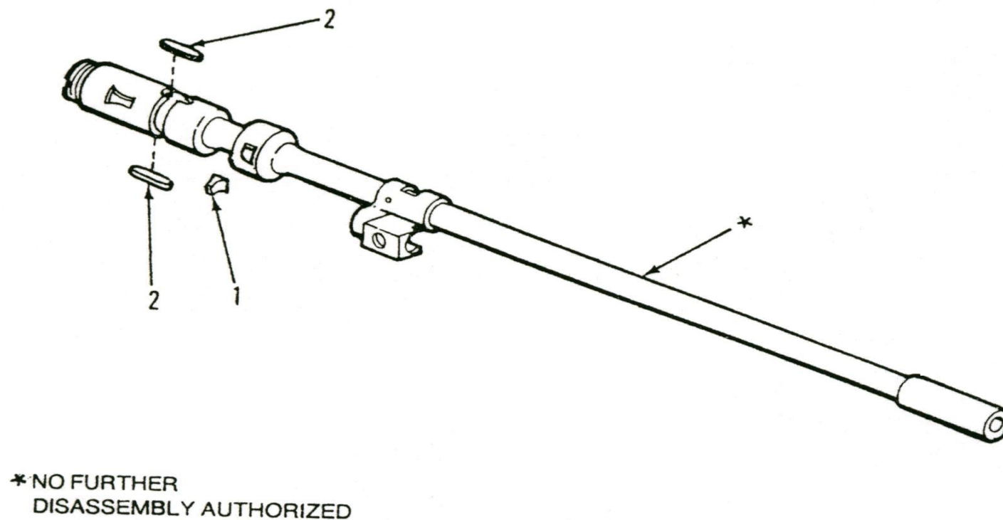
Figure 11. Barrel assembly.
