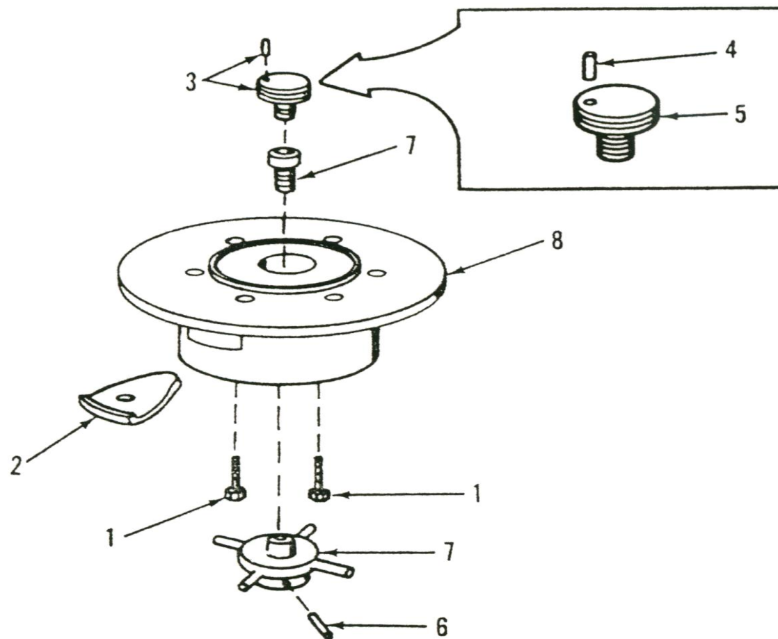
Figure 28. Rifle mount adapter assembly and collar and pin assembly.
