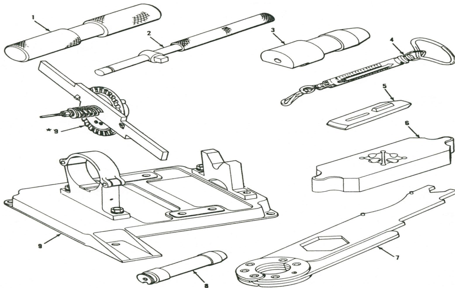
Figure 33. Special tools.
