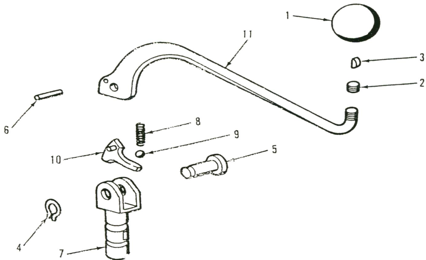
Figure 17. Breechblock operating lever.
