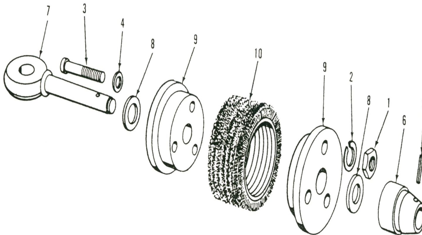
Figure 32. Artillery cleaning brush.
