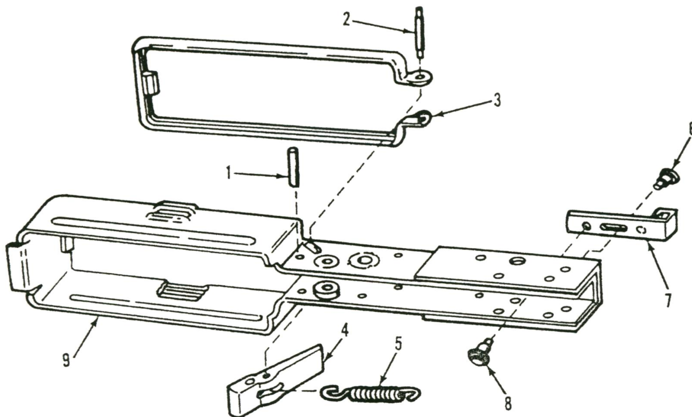
Figure 8. Housing and catch assembly.
