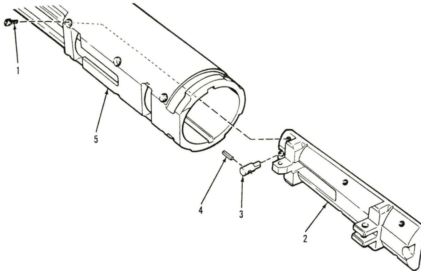
Figure 10. Receiver assembly.
