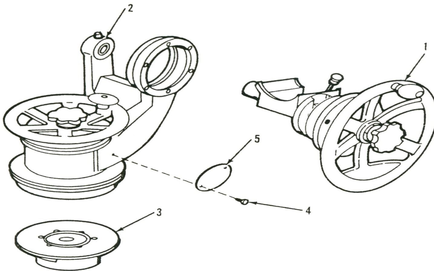
Figure 27. Mount, rifle, 106-mm: M92.
