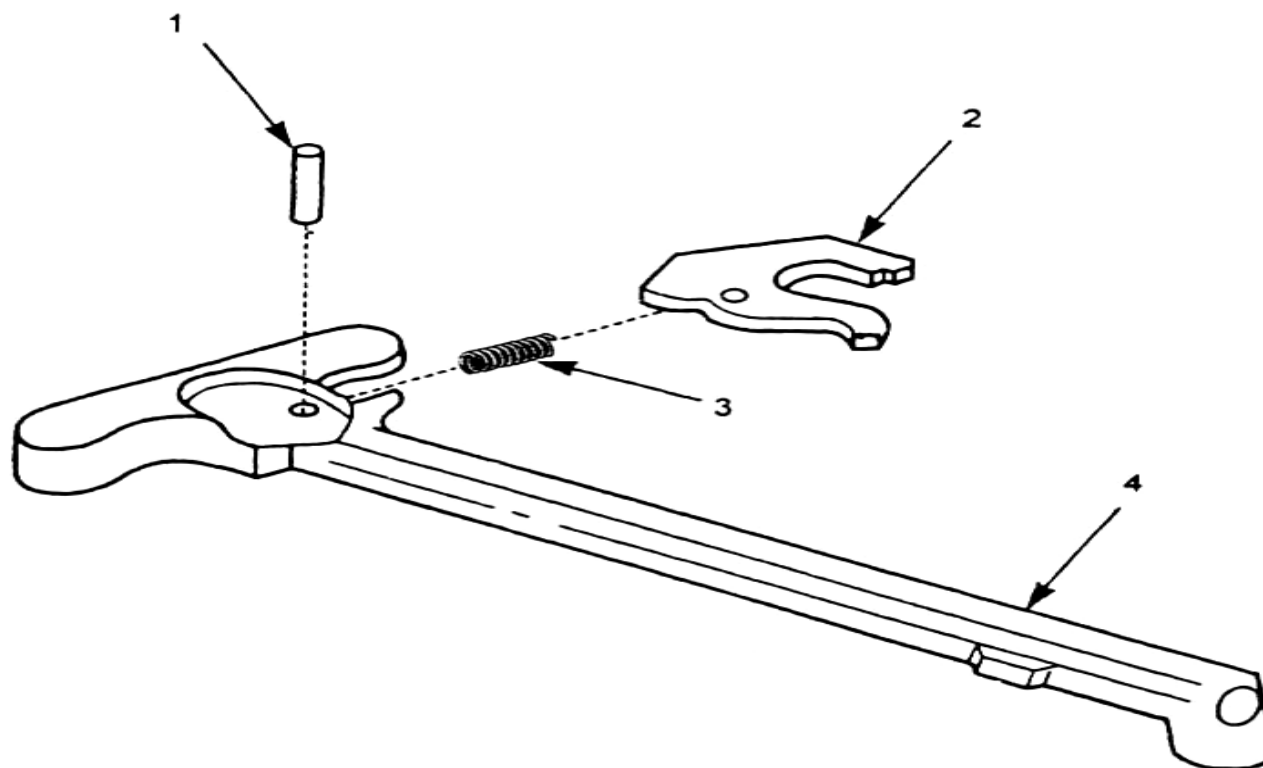
Handle Assembly 8448517.
