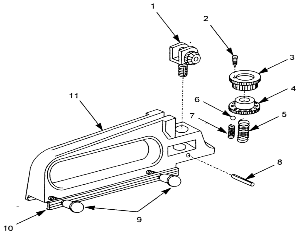
Carrying Handle Assembly (M16A4, M4, M4A1) 12951011
