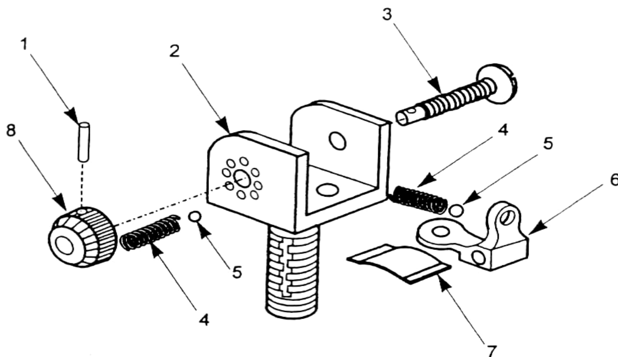
Rear Sight Assembly (M16A4, M4 and M4A1) 12951026.
