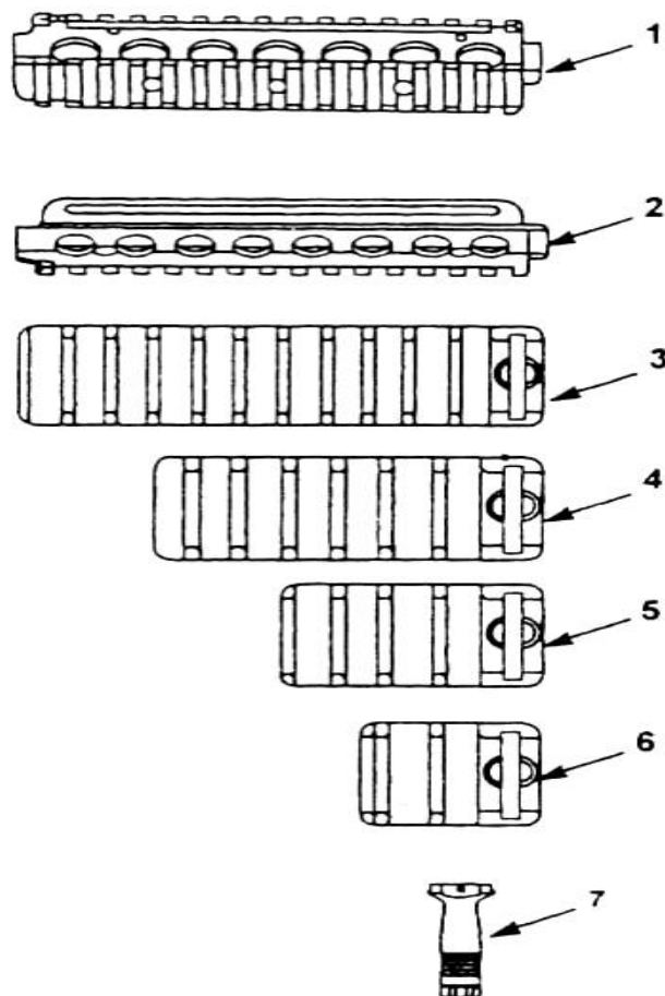
(M4 and M4A1) M4 Adapter Rail, Weapon Mounted 12973095.
