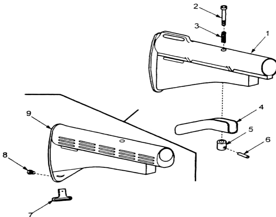
Buttstock Assembly (M4 and M4A1) 9390012 (Current) 12012082 (New).
