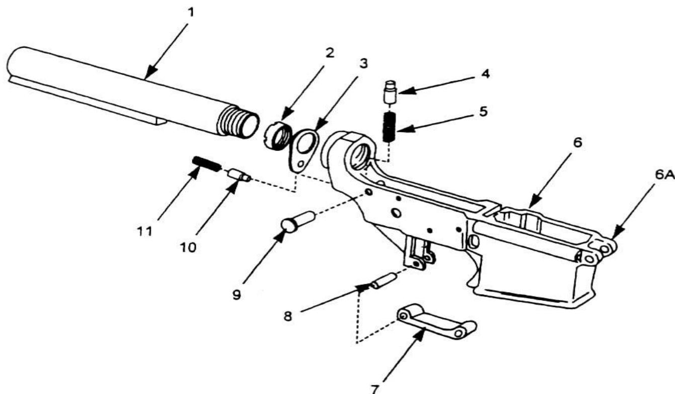
Lower Receiver and Receiver Extension Assembly (M4) 9390011 and (M4A1) 12972690
