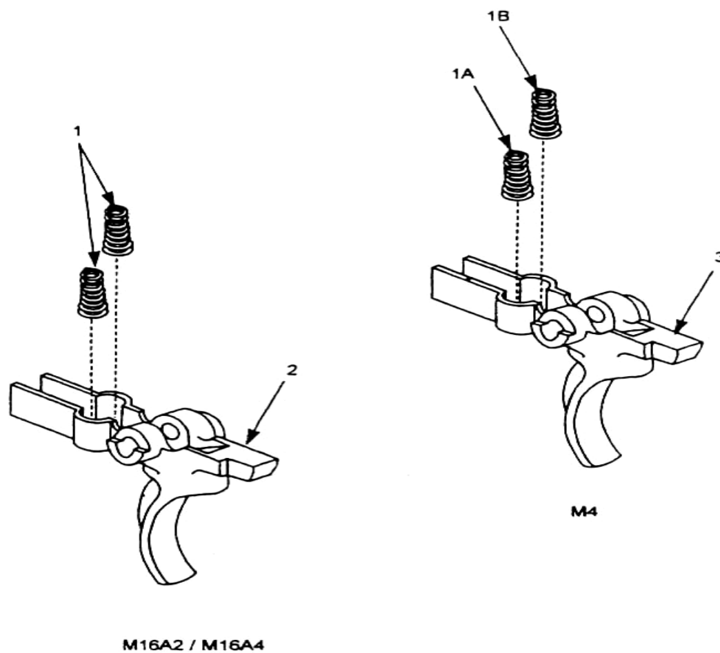
Trigger Subassembly (M16A2, M16A4) 9392518 and (M4) 12972696.
