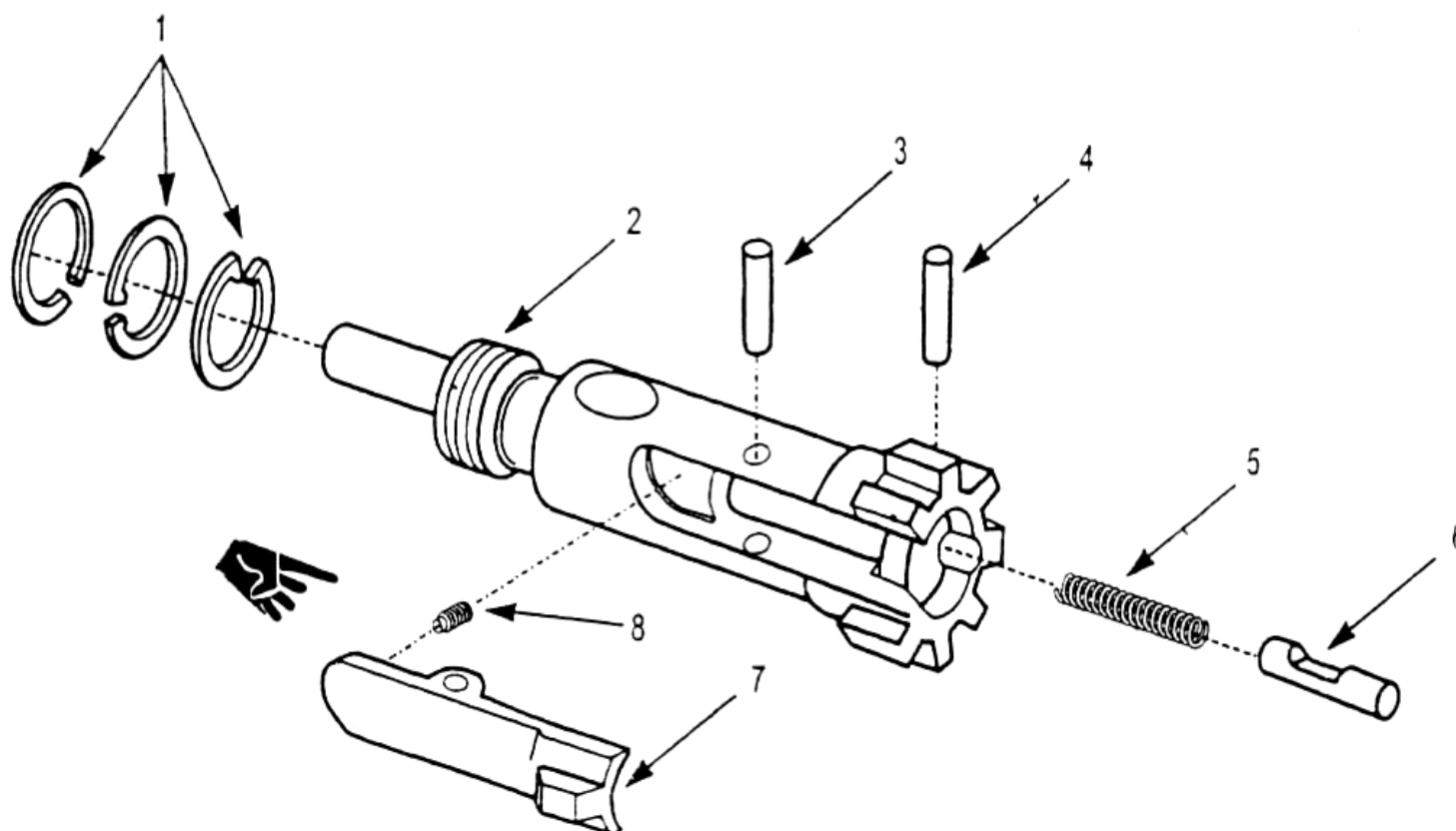
Bolt Assembly 12972691.
