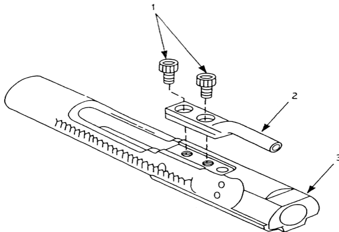
Key and Bolt Carrier Assembly 8448505.
