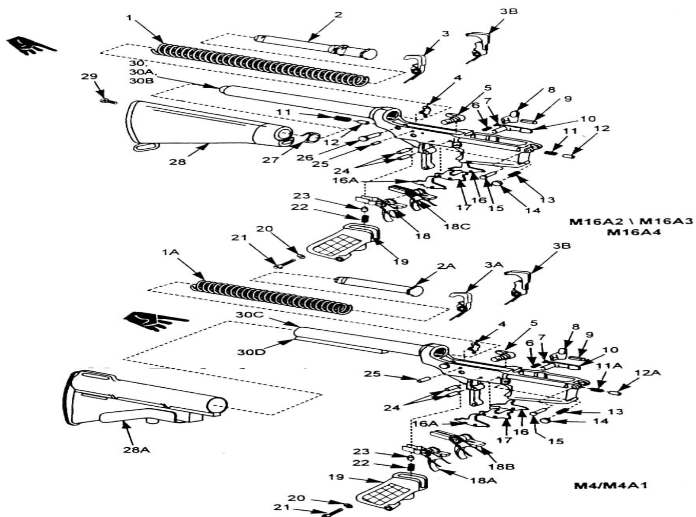
Lower Receiver and Buttstock Assembly (M16A2) 9349100, (M16A3) 12012001, (M16A4) 12598101, (M4) 9390011 and (M4A1) 12972690.
