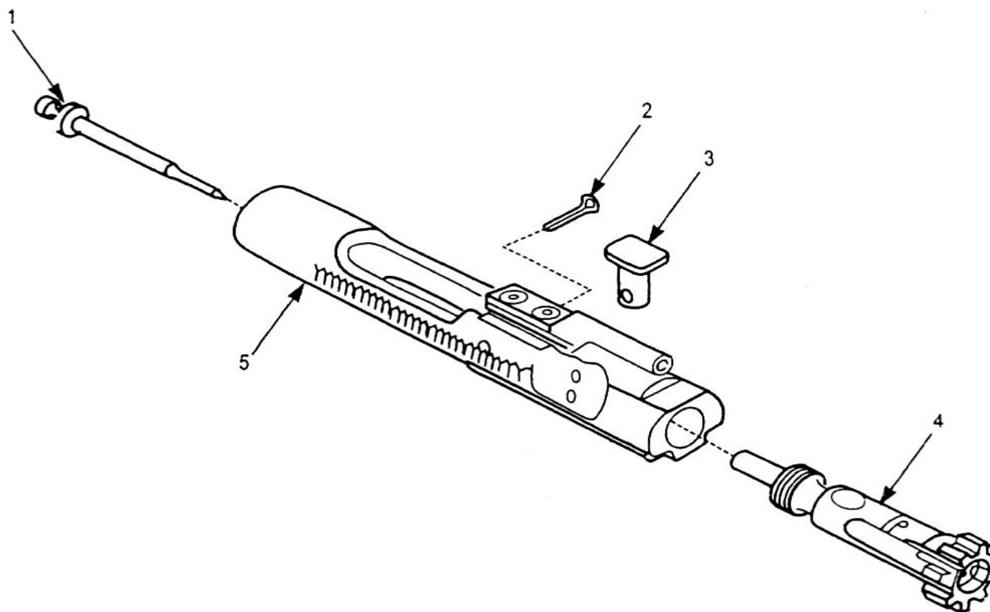
Bolt and Bolt Carrier Assembly 12011849.
