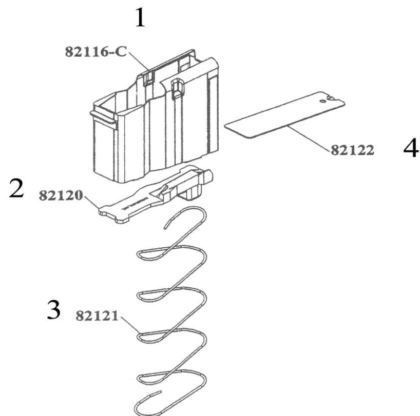
82116-A MAGAZINE ASSEMBLY
