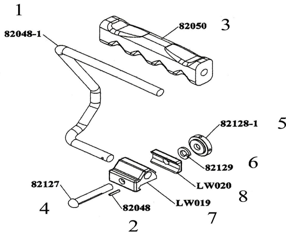
LW019-A1 CARRYING HANDLE ASSEMBLY
